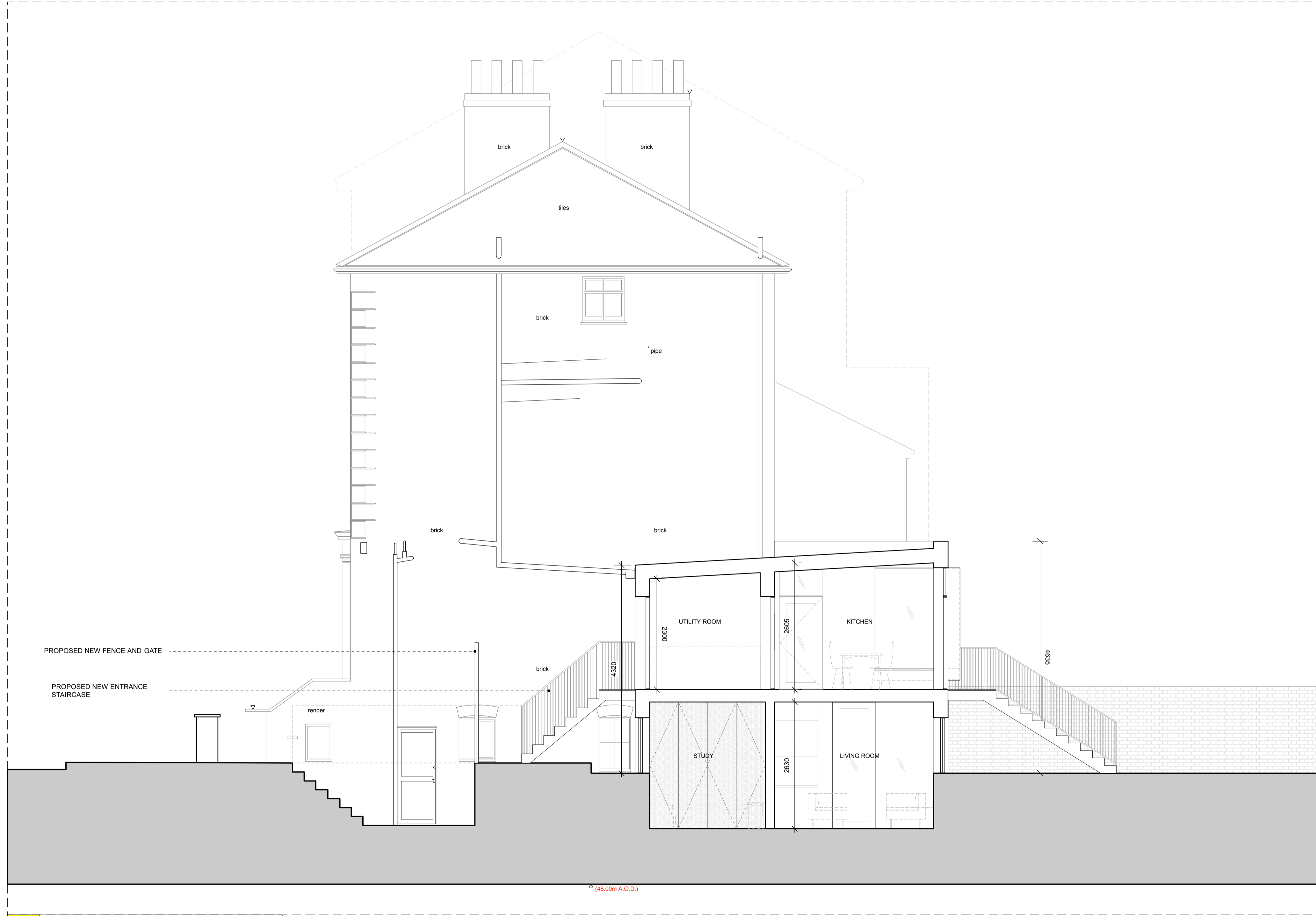
01 PROPOSED SECTION CC 1:50 @ A1, 1:100 @ A3
