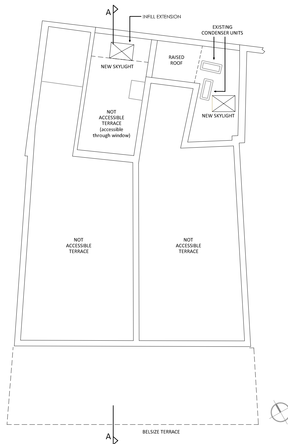
ROOF PLAN SCALE 1:100@A3 / 1:50@A1
