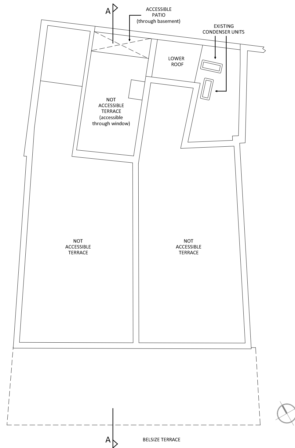
ROOF PLAN SCALE 1:100@A3 / 1:50@A1
