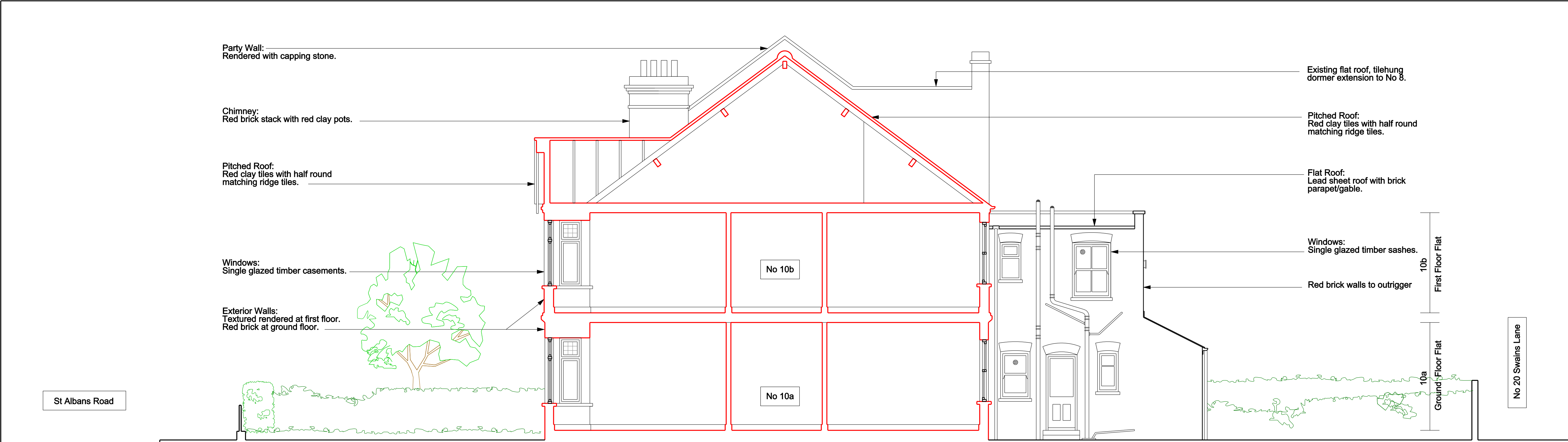
Existing Section AA
