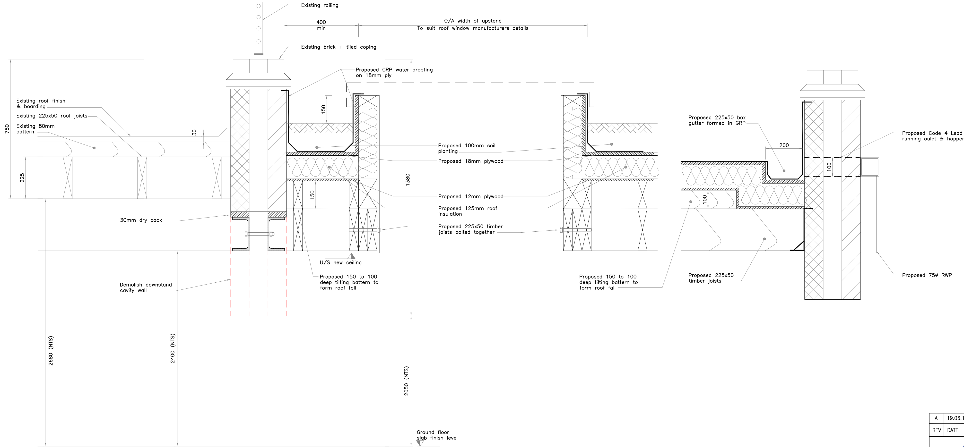
SECTION A-A Scale 1:10
