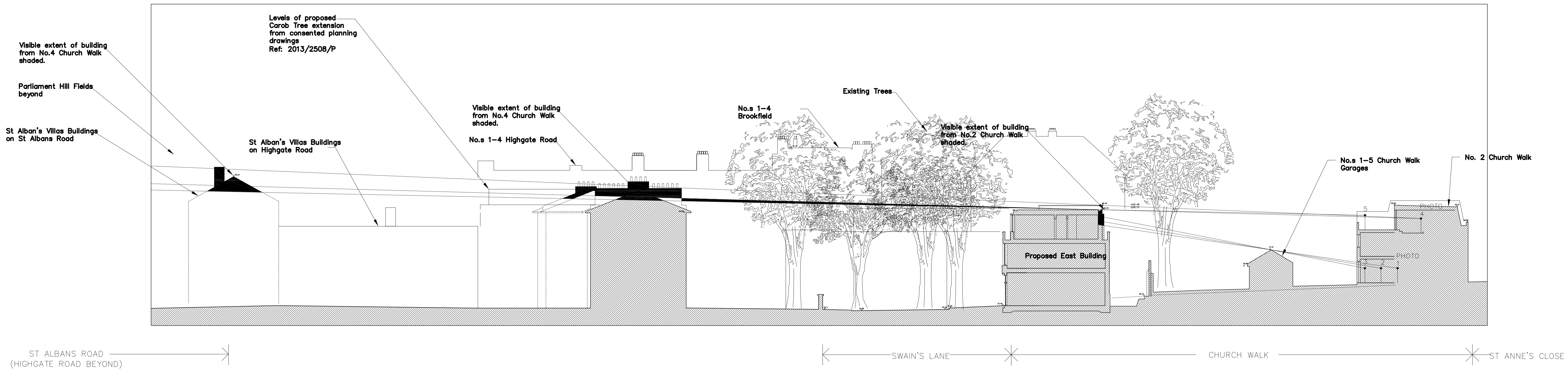
SECTION E-E
