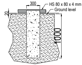
CROSS SECTION B-B
