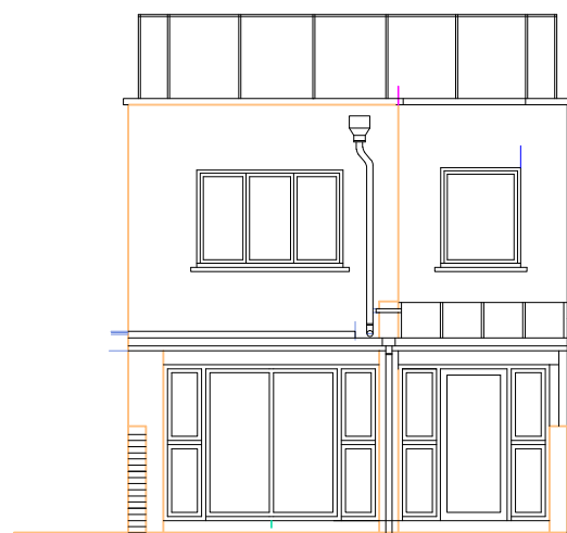
PROPOSED REAR ELEVATIONS
