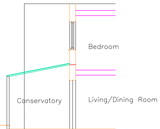
EXISTING SECTION
