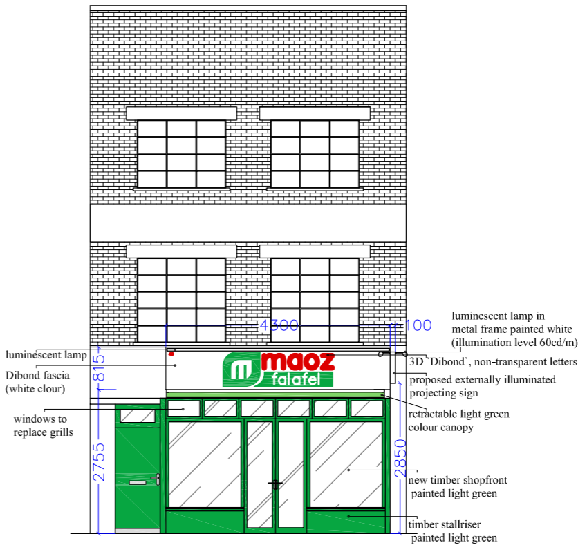
FRONT ELEVATION WITH FOLDED CANOPY (as proposed)
