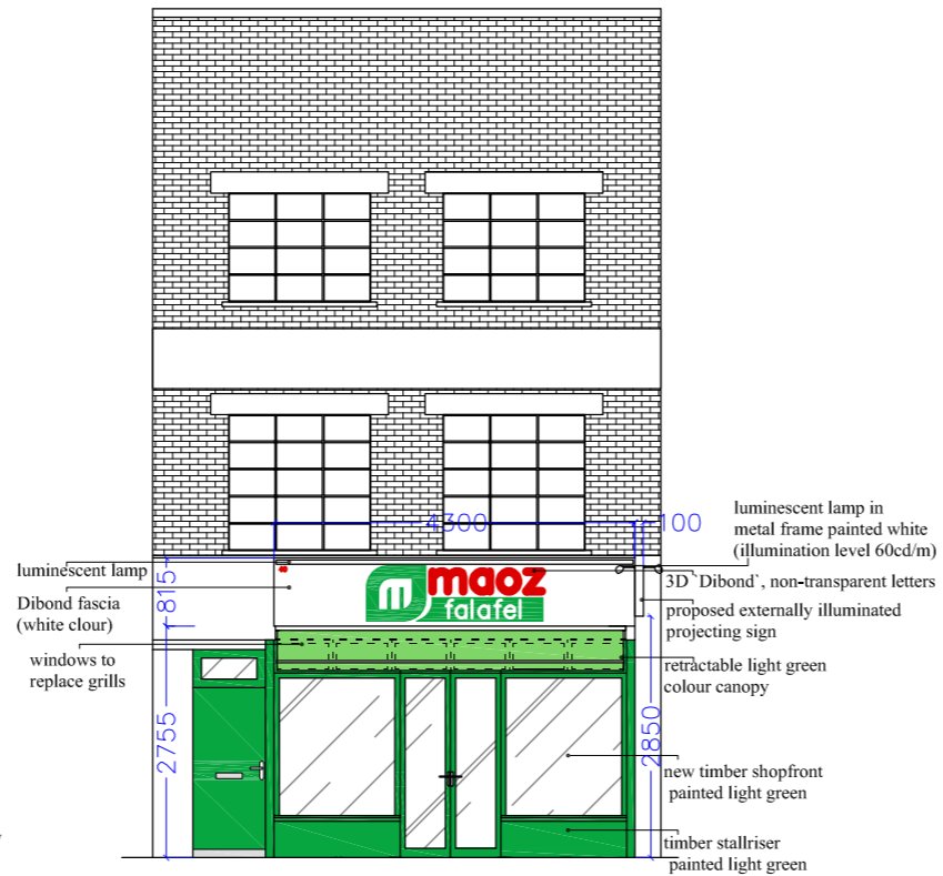
FRONT ELEVATION (as proposed)
