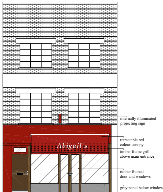
FRONT ELEVATION (as existing)
