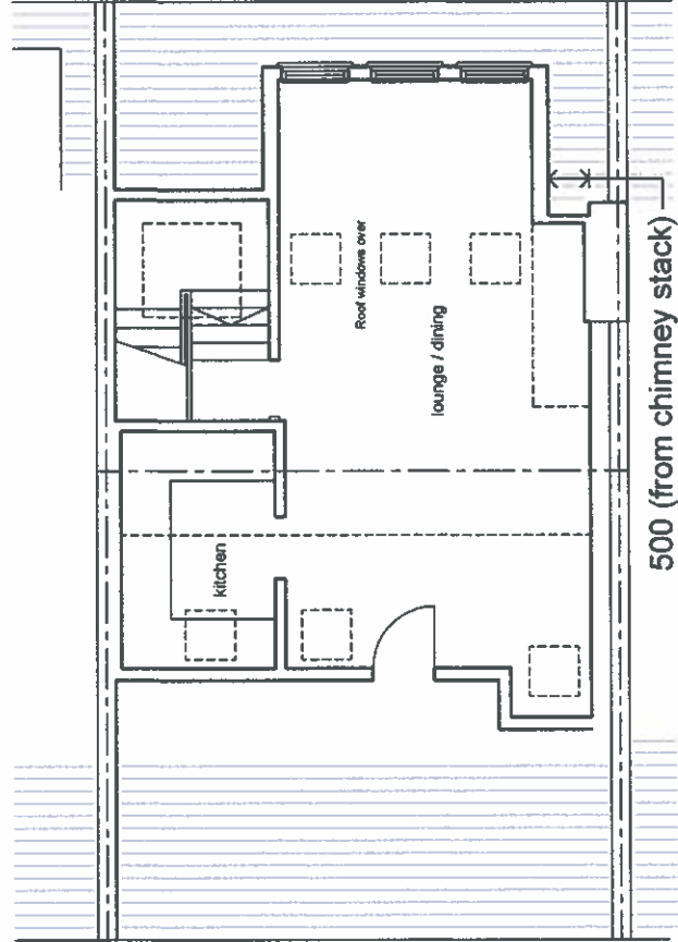
third floor
