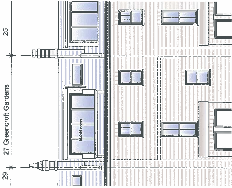
existing elevation
