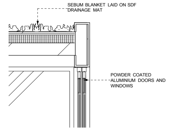
DETAIL_1:20
