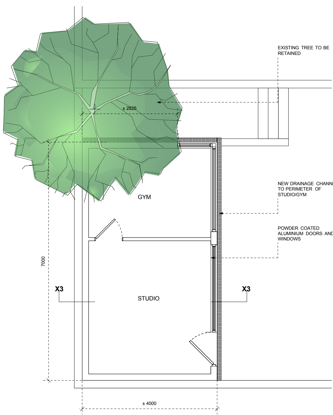
PLAN
