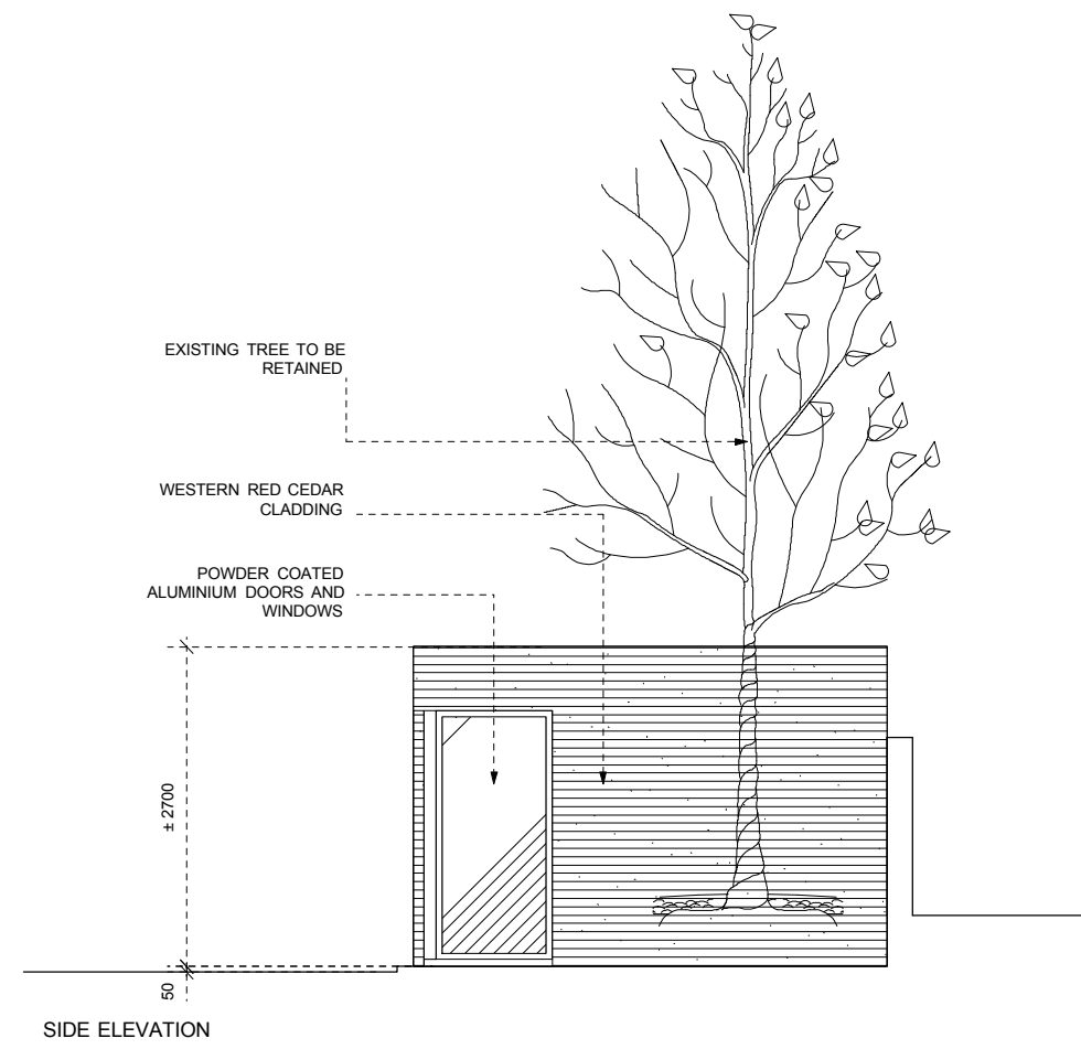
SIDE ELEVATION
