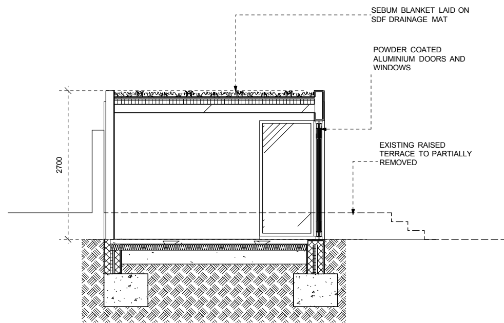
SECTION X3
