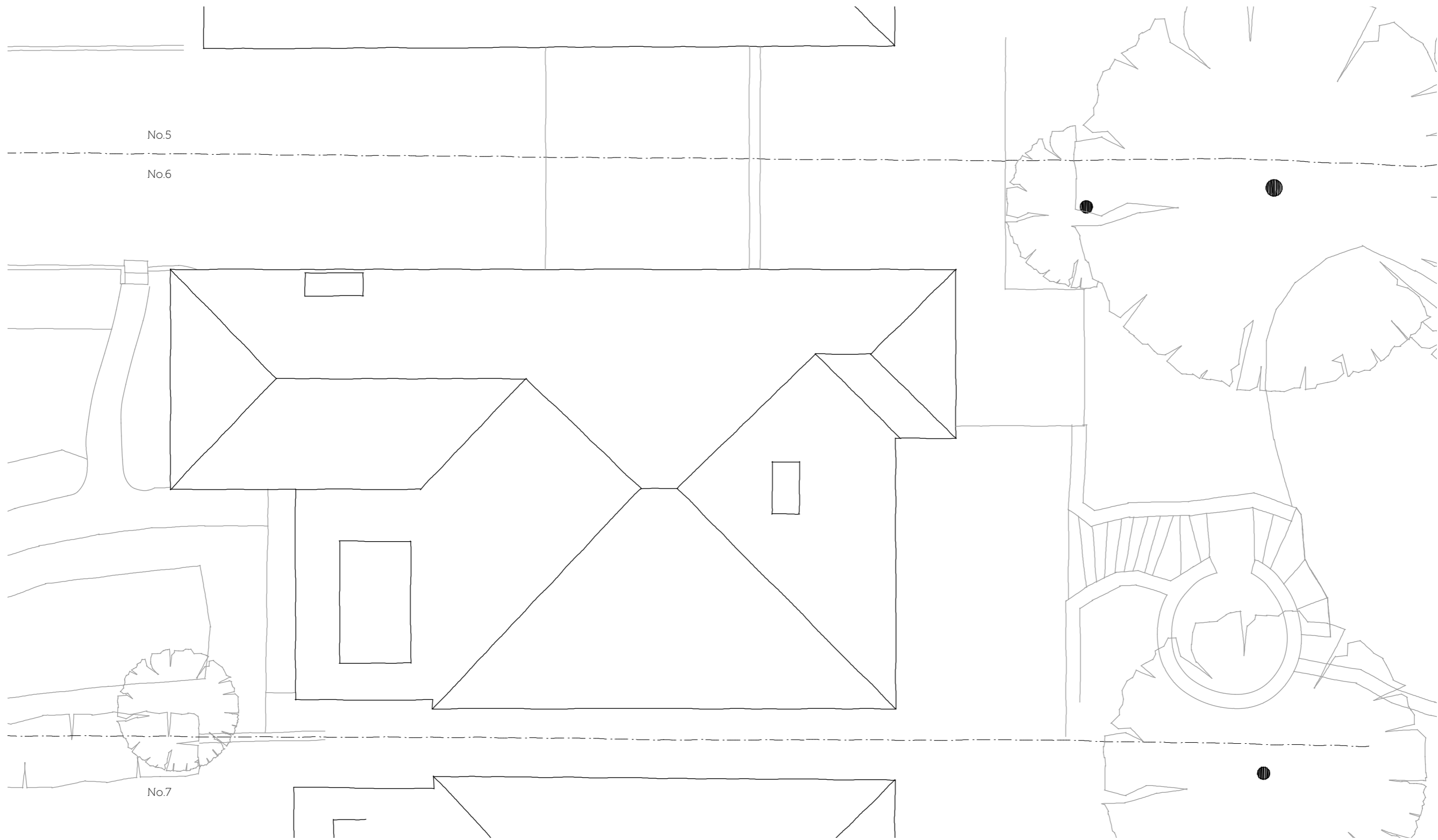
Roof plan
