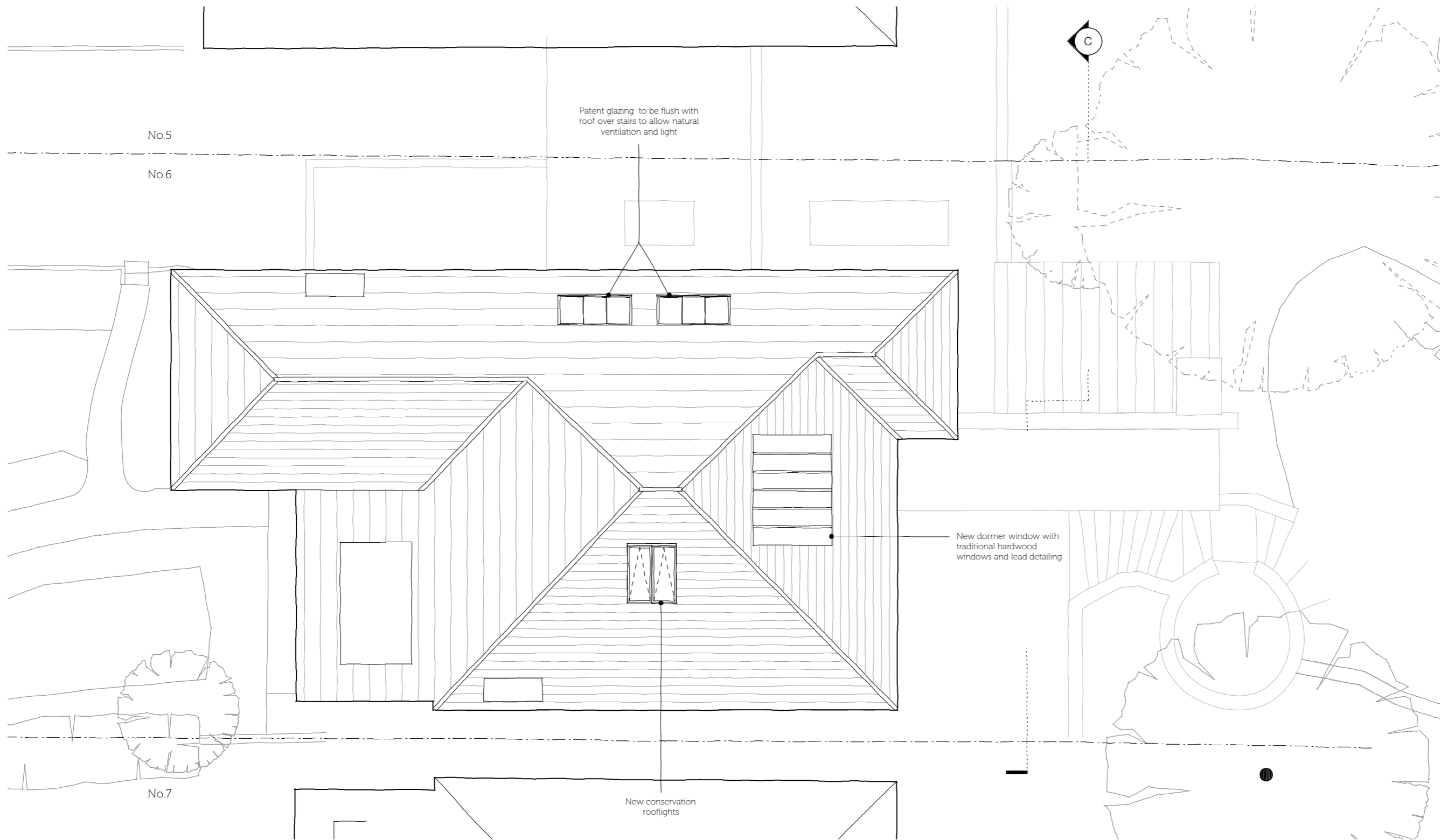
Roof plan
