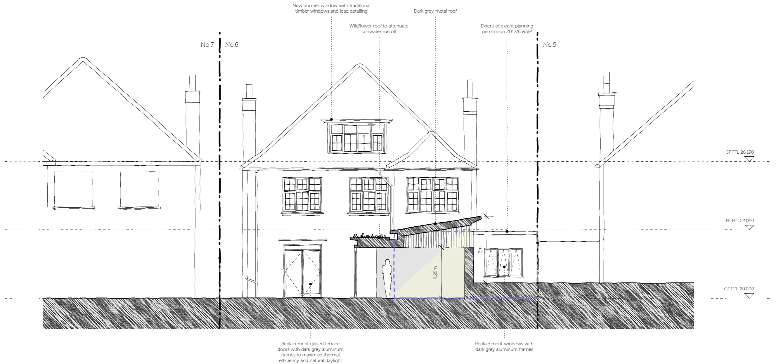
Section CC
