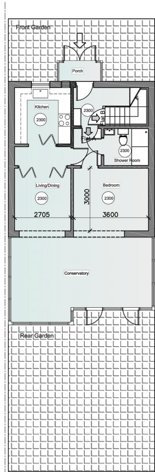
Proposed Ground Floor Plan Scale 1:100
