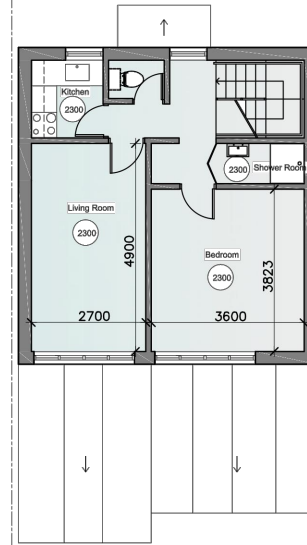
Proposed First Floor Plan Scale 1:100
