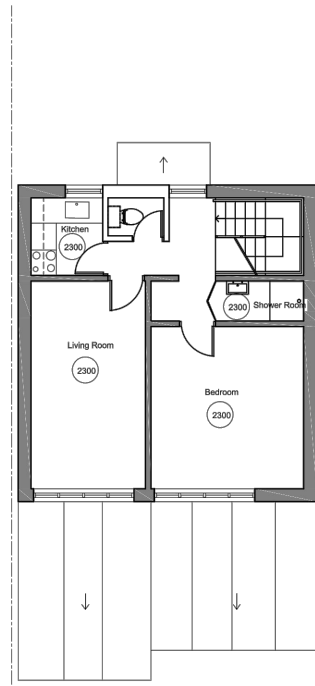
Existing First Floor Plan Scale 1:100
