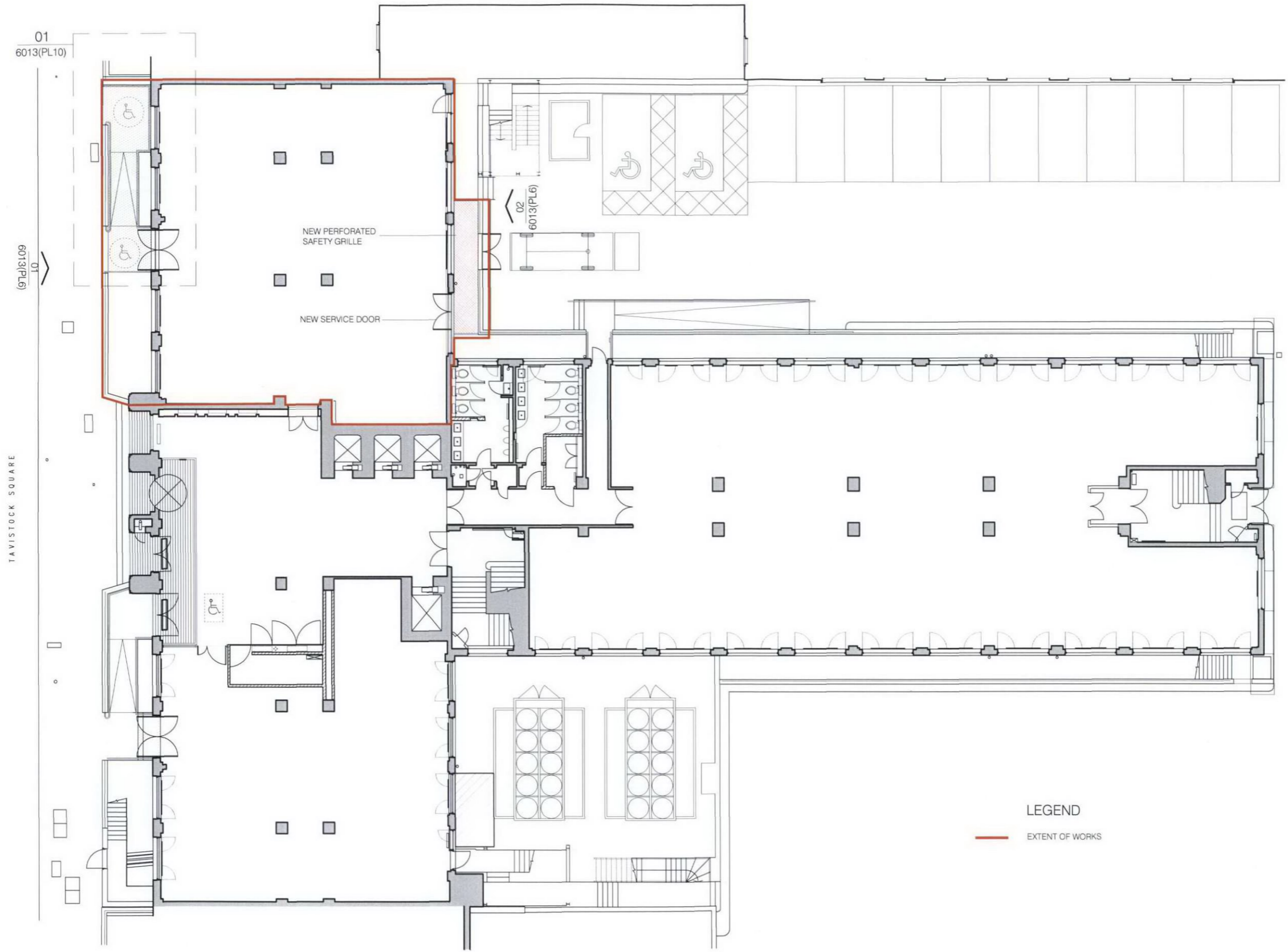
1 PROPOSED GROUND FLOOR PLAN SCALE 1:200
