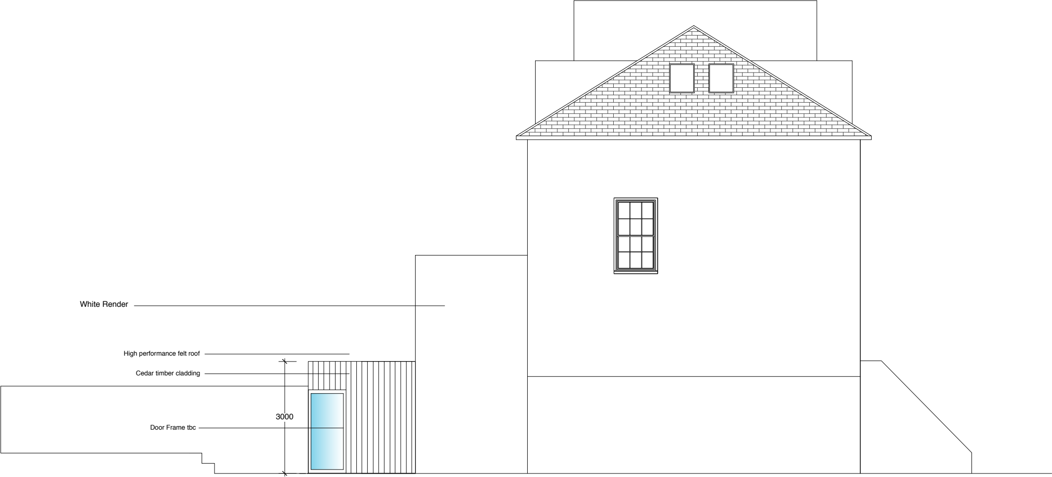
1 111 Elevation: Side Elevation: Proposed Scale: 1:100 @ A3
