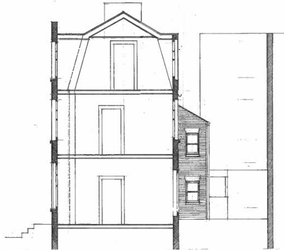
Section proposed
