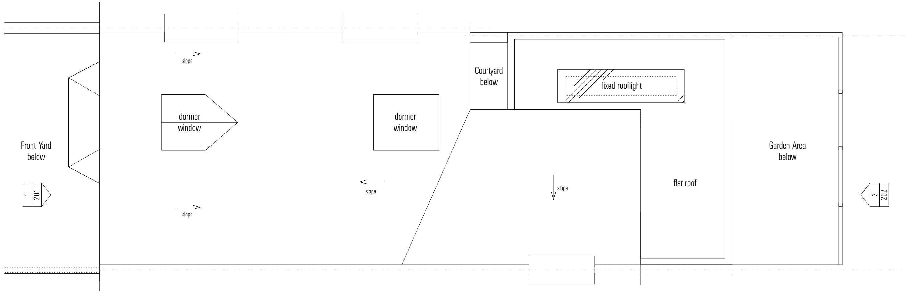
ROOF PLAN
