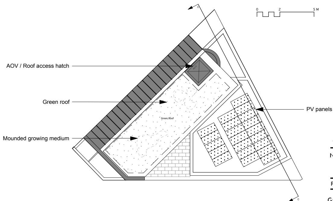
Roof Plan
