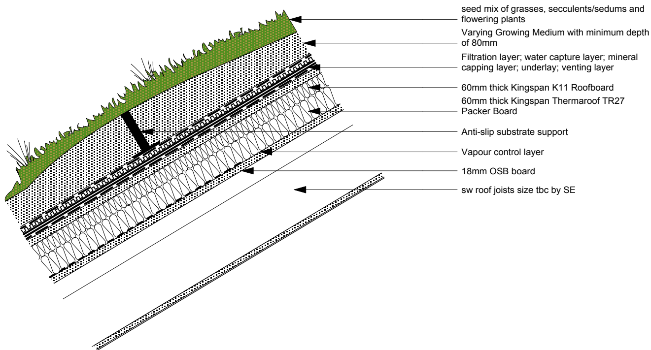
Detail section
