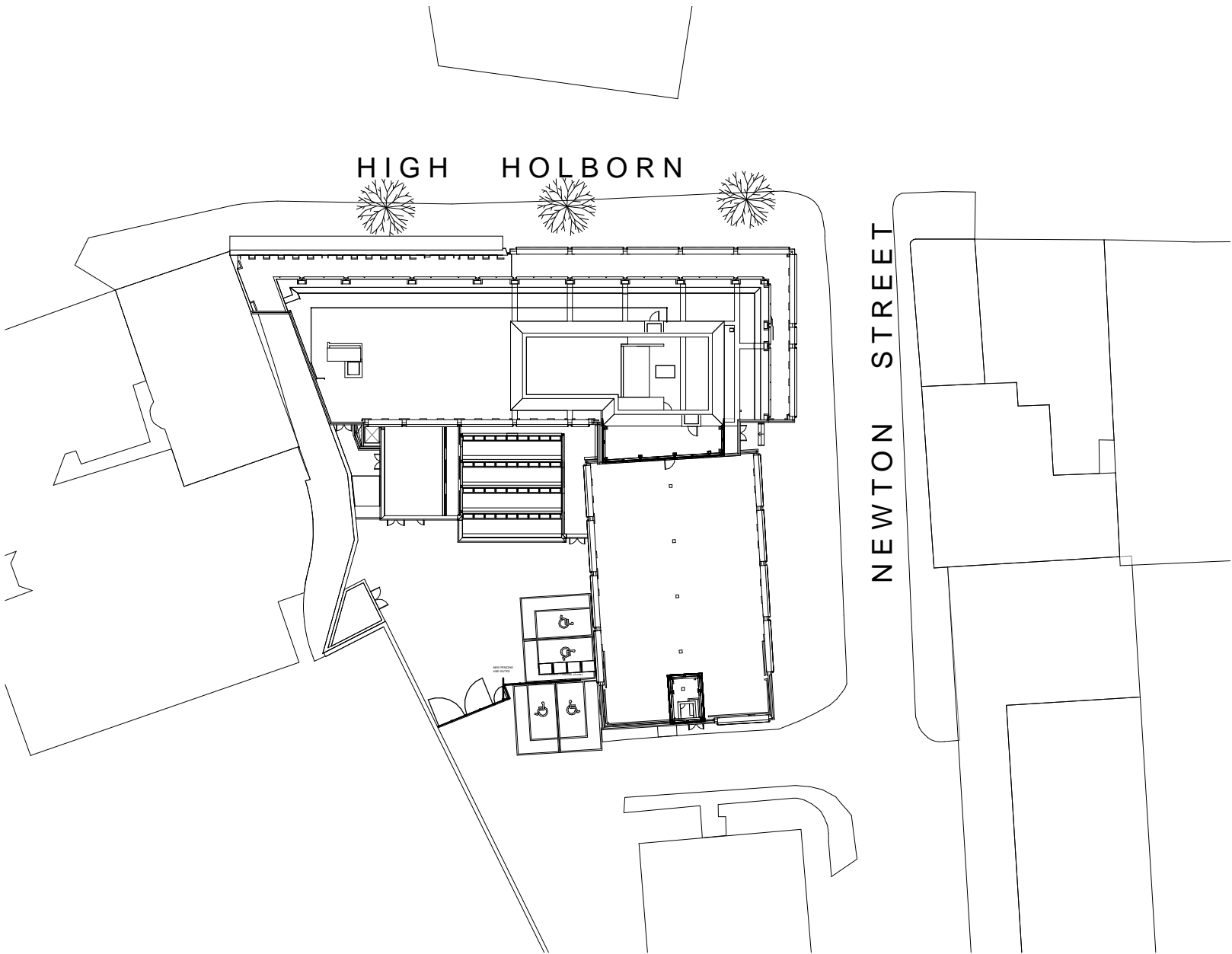
RETAIL UNIT - SITE PLAN (PROPOSED) 1 : 500
