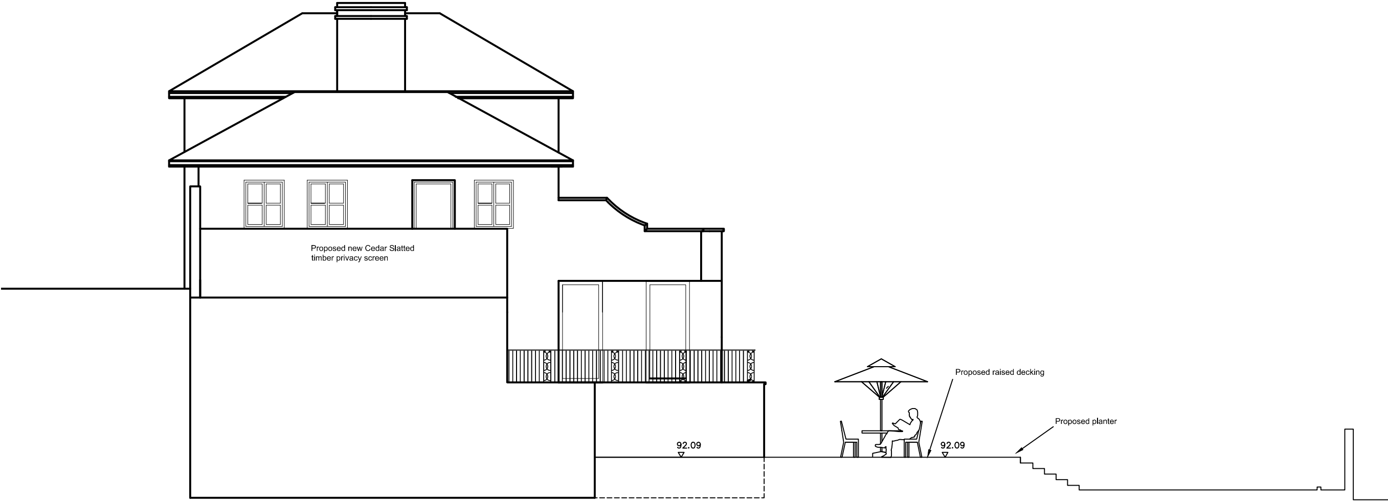
PROPOSED WEST ELEVATION (WITHOUT FOLIAGE) SCALE 1:100
