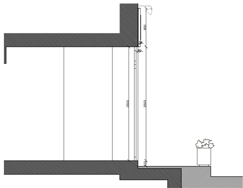
PROPOSED SECTION THROUGH ENTRANCE _ Scale 1/50
