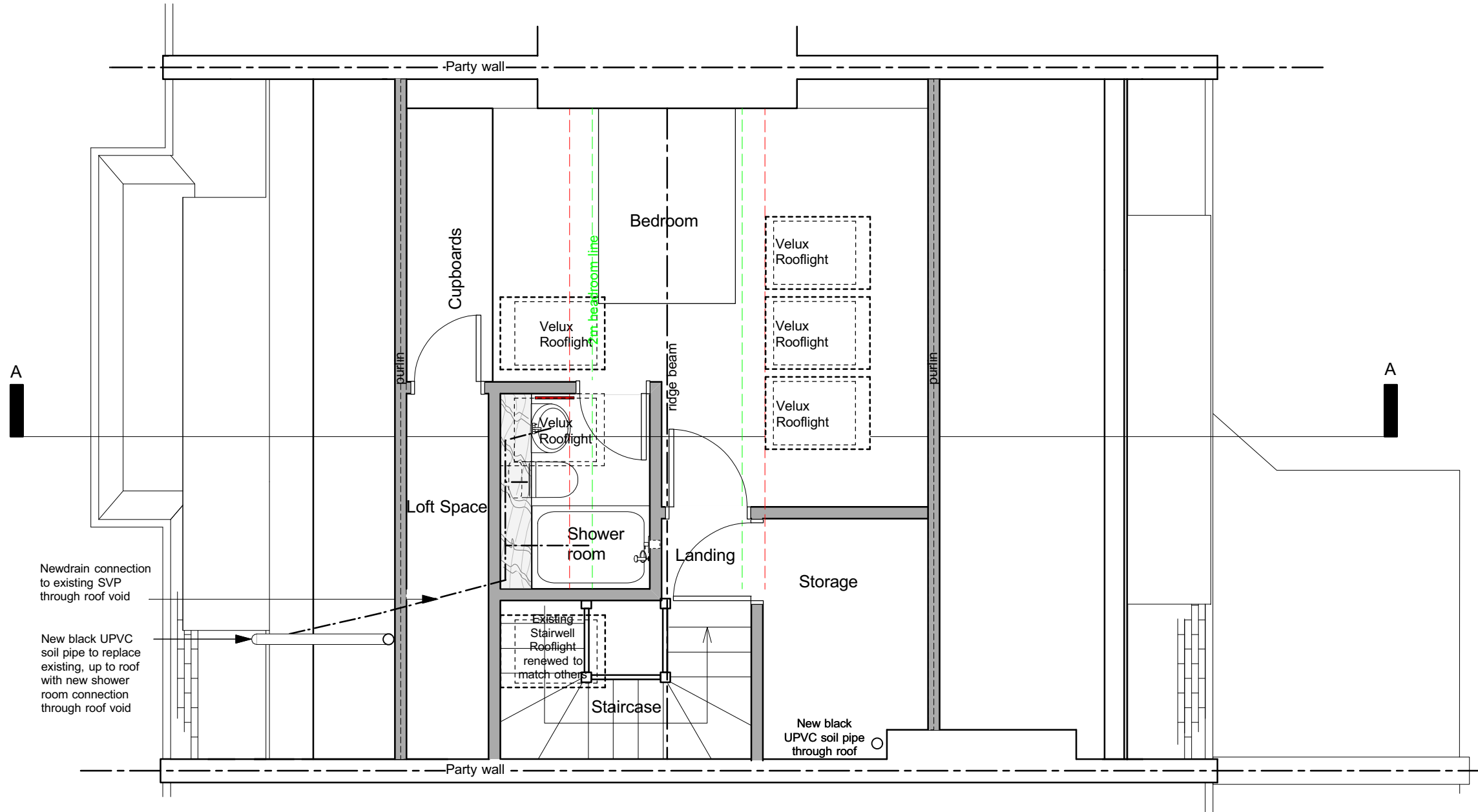
PROPOSED DORMER LOFT FLOOR PLAN
