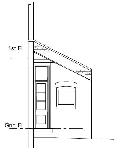
EXISTING SIDE ELEVATION of CLOSET WING of No. 4
