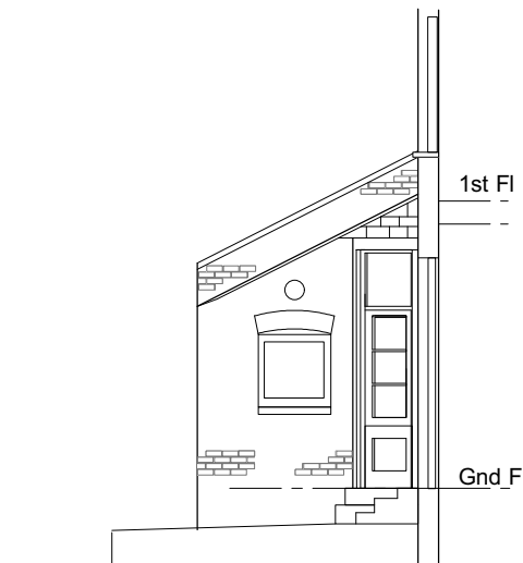
EXISTING SIDE ELEVATION of CLOSET WING of No. 6
