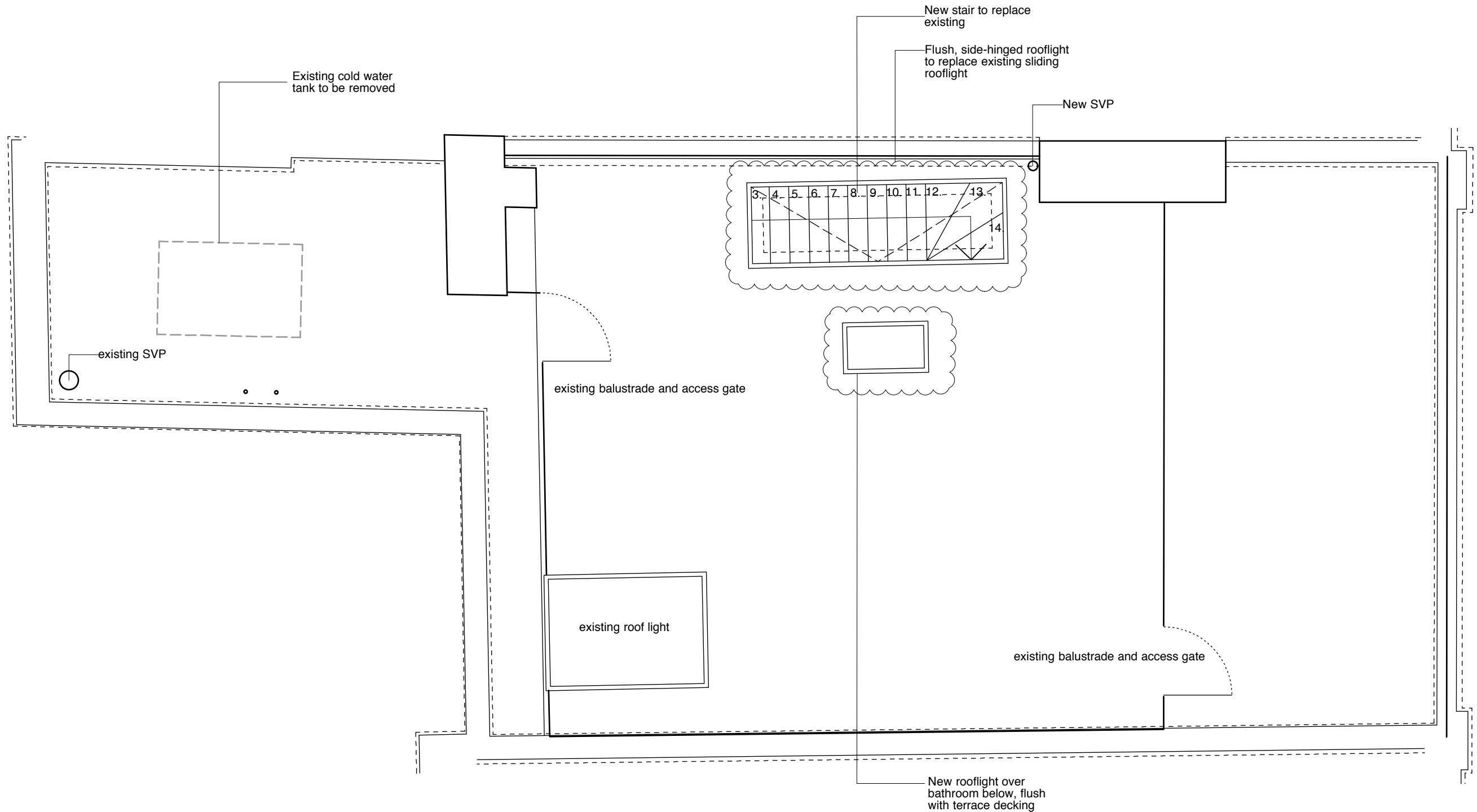
A Proposed Terrace Roof Plan
