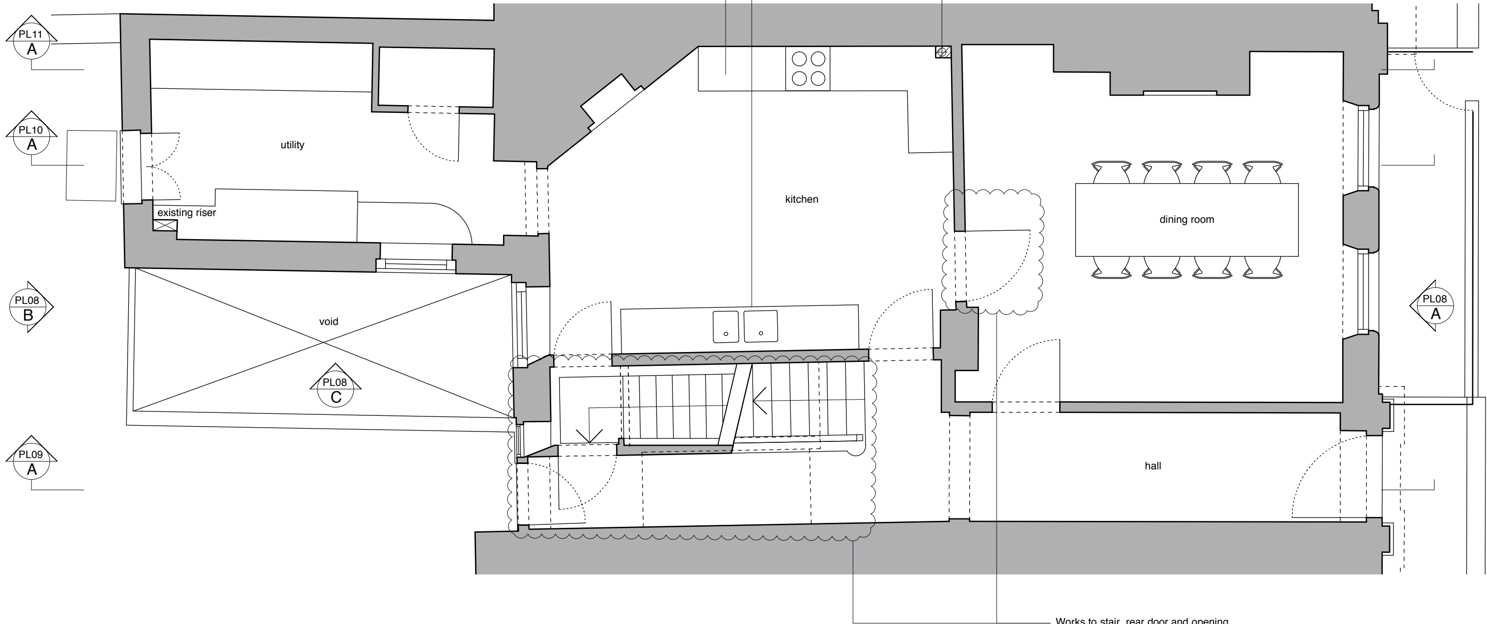
A Proposed Ground Floor Plan
