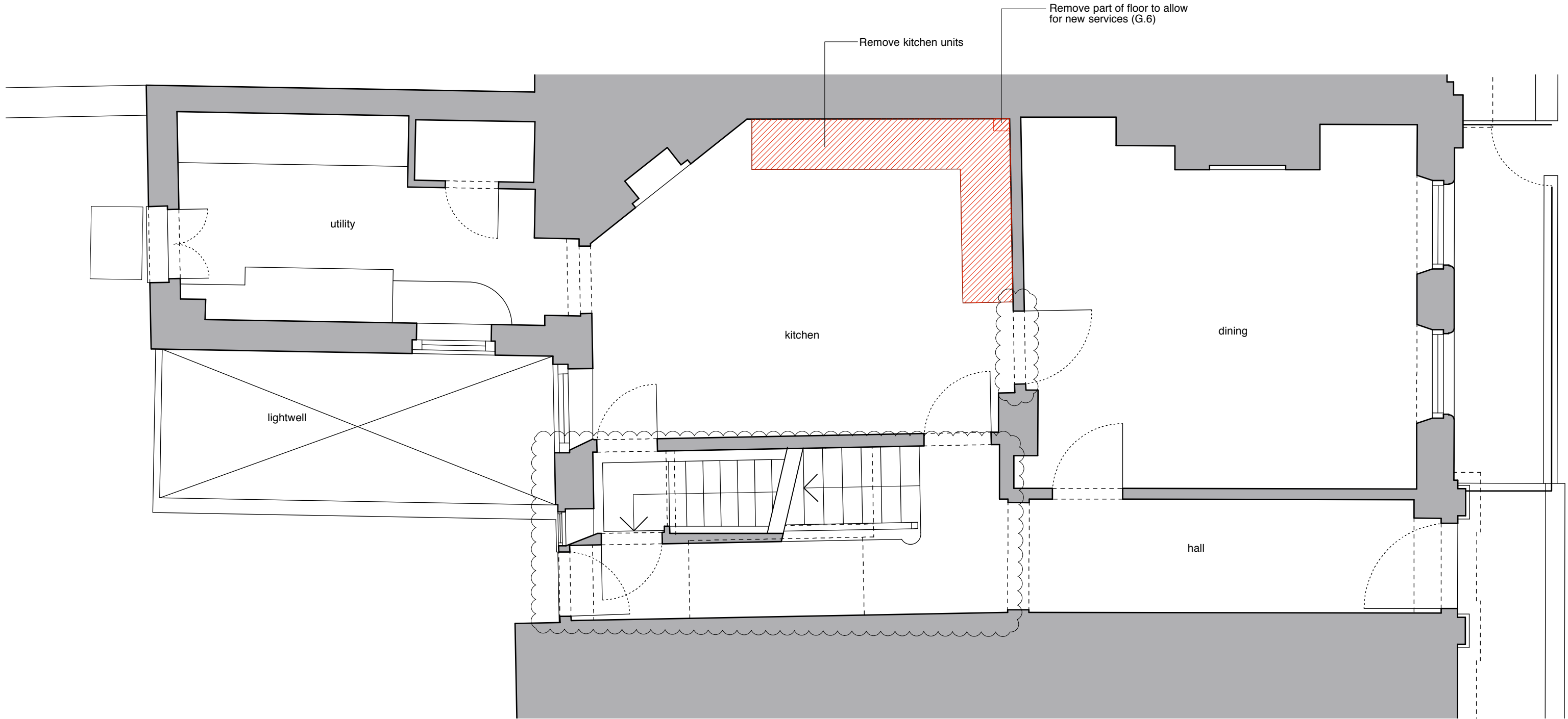
A Ground Floor Demolition Plan
