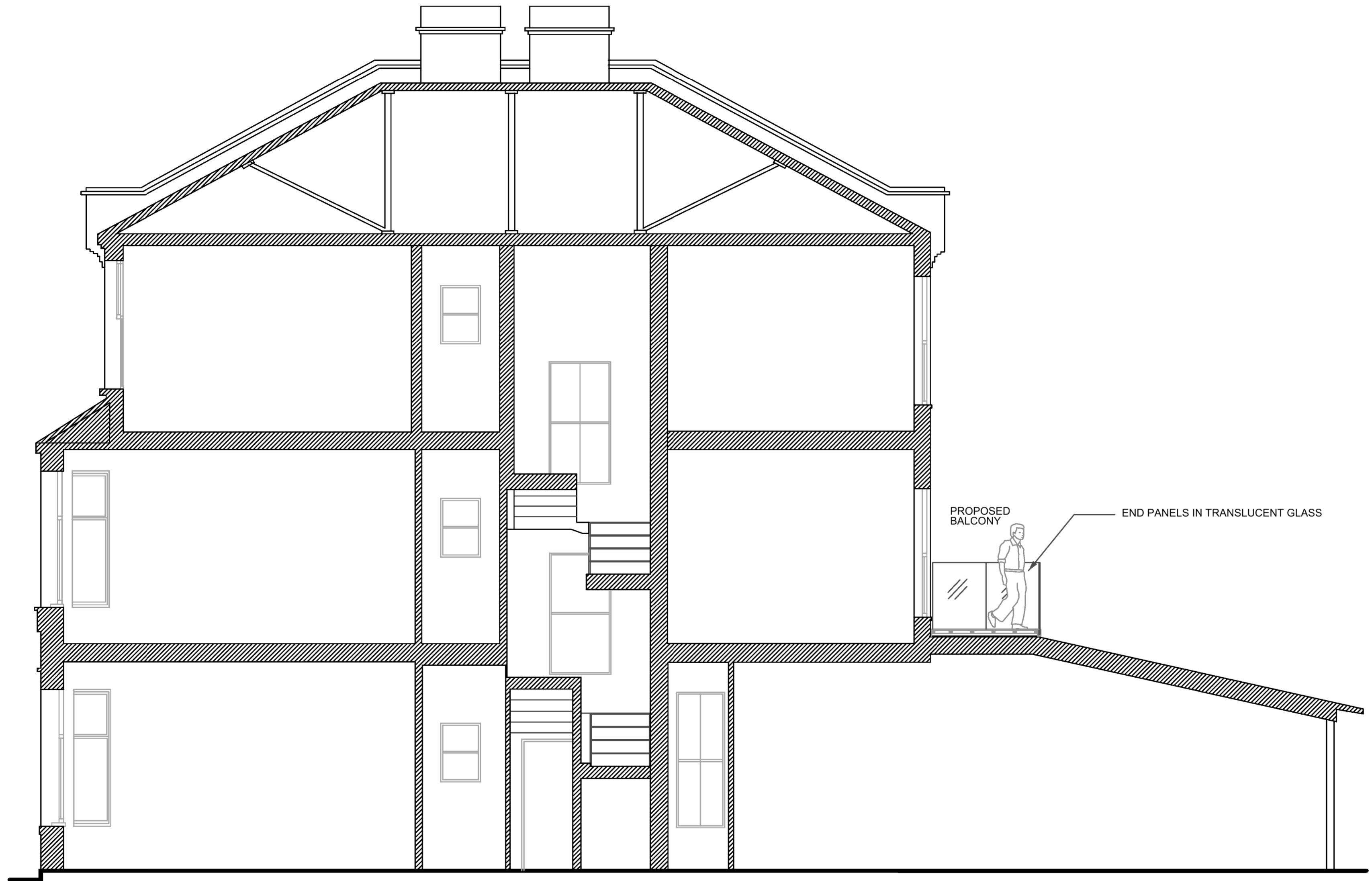
PROPOSED SECTION L/06
