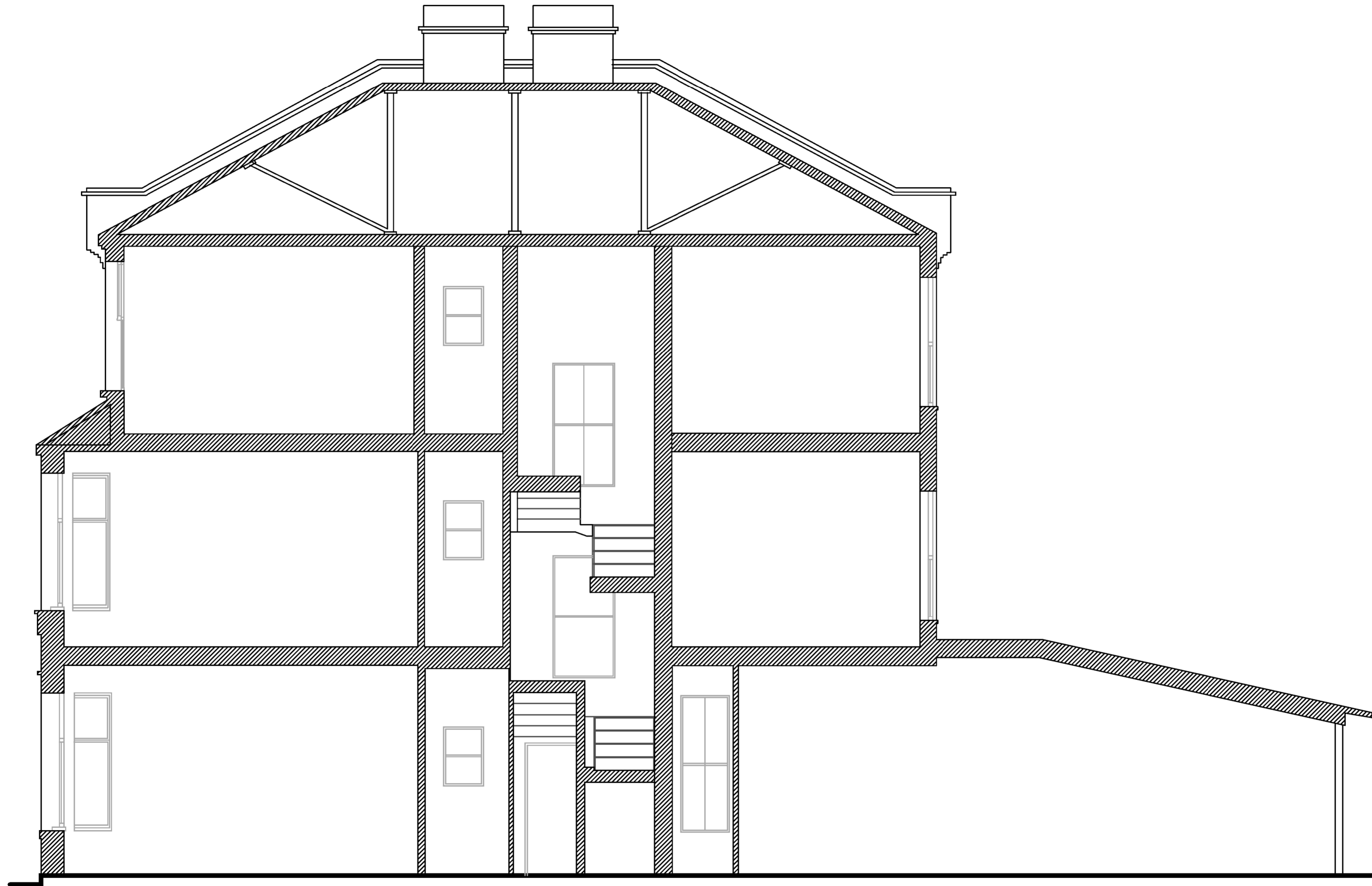
EXISTING SECTION L/03
