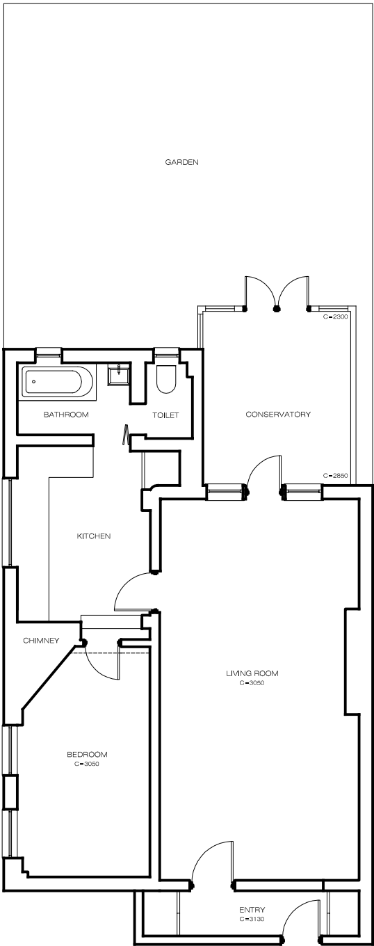
EXISTING GROUND FLOOR SCALE 1:100
