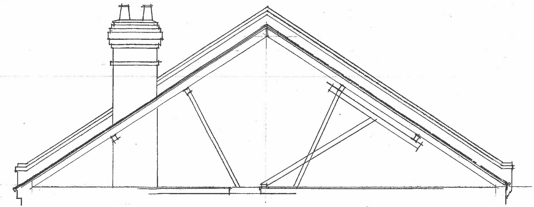
ROOF SECTION
