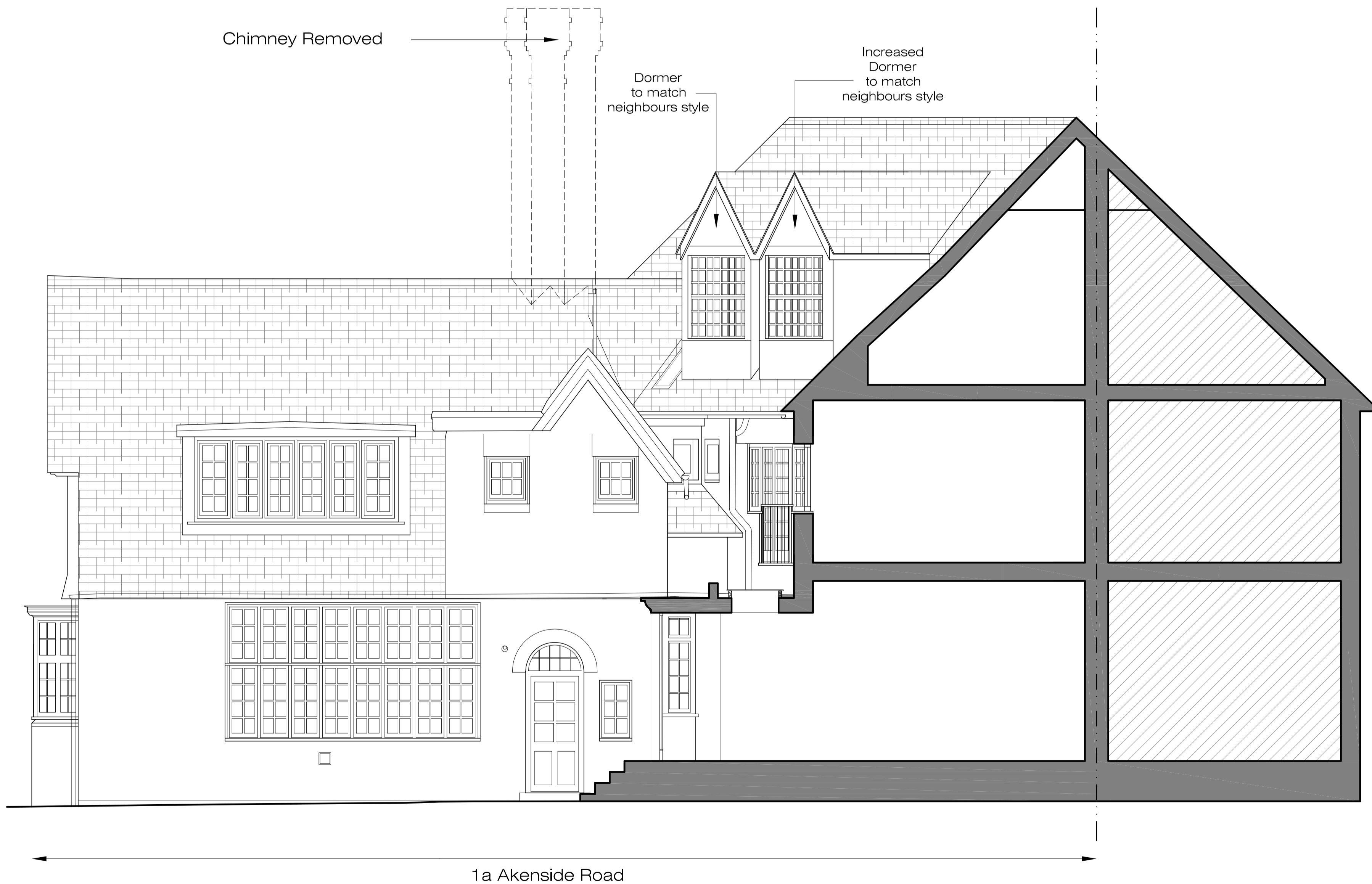
PROPOSED REAR ELEVATION/SECTION 01 SCALE 1:100@A3 PA-07
