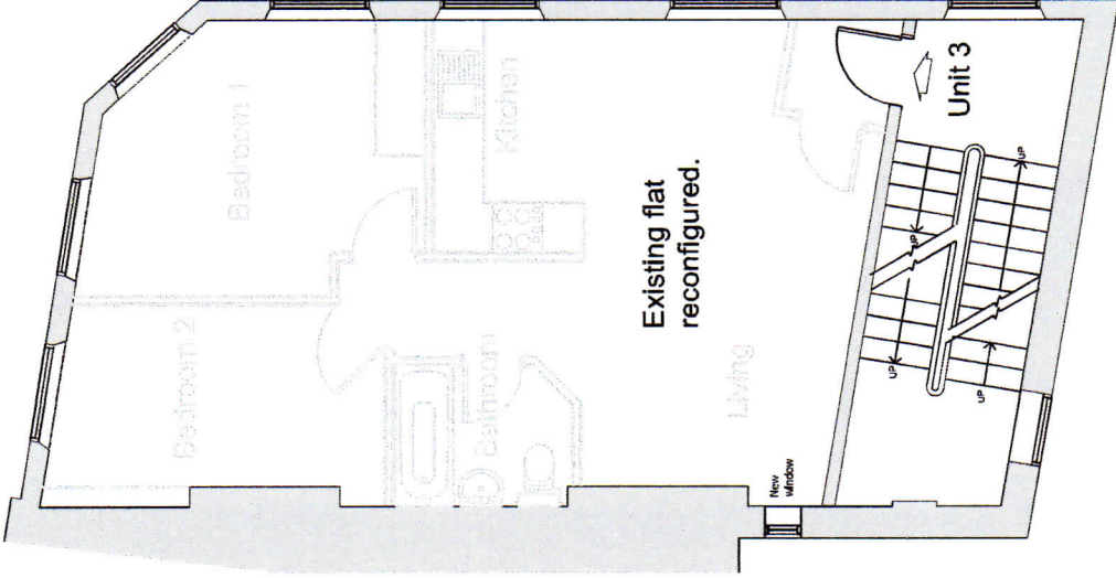
APPROVED SF Plan 1:100
