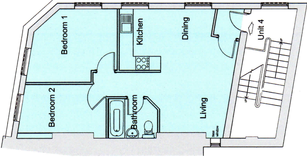
APPROVED TF Plan 1:100
