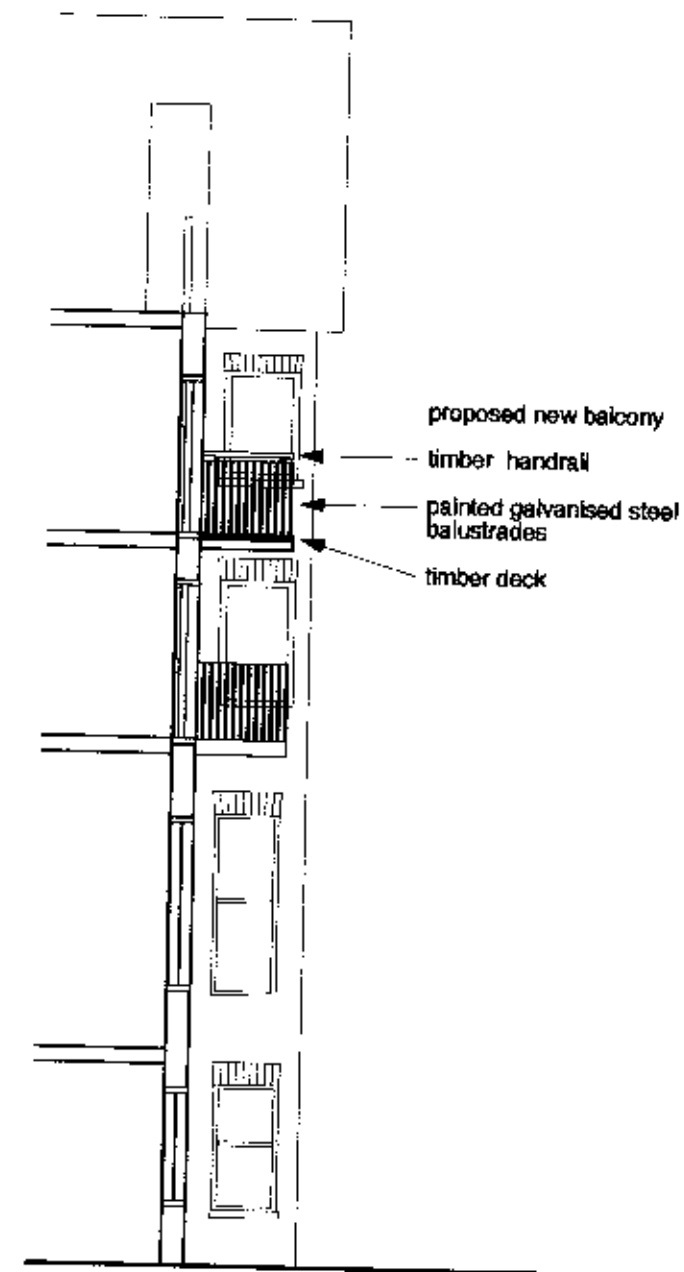
SECTION 1:100
