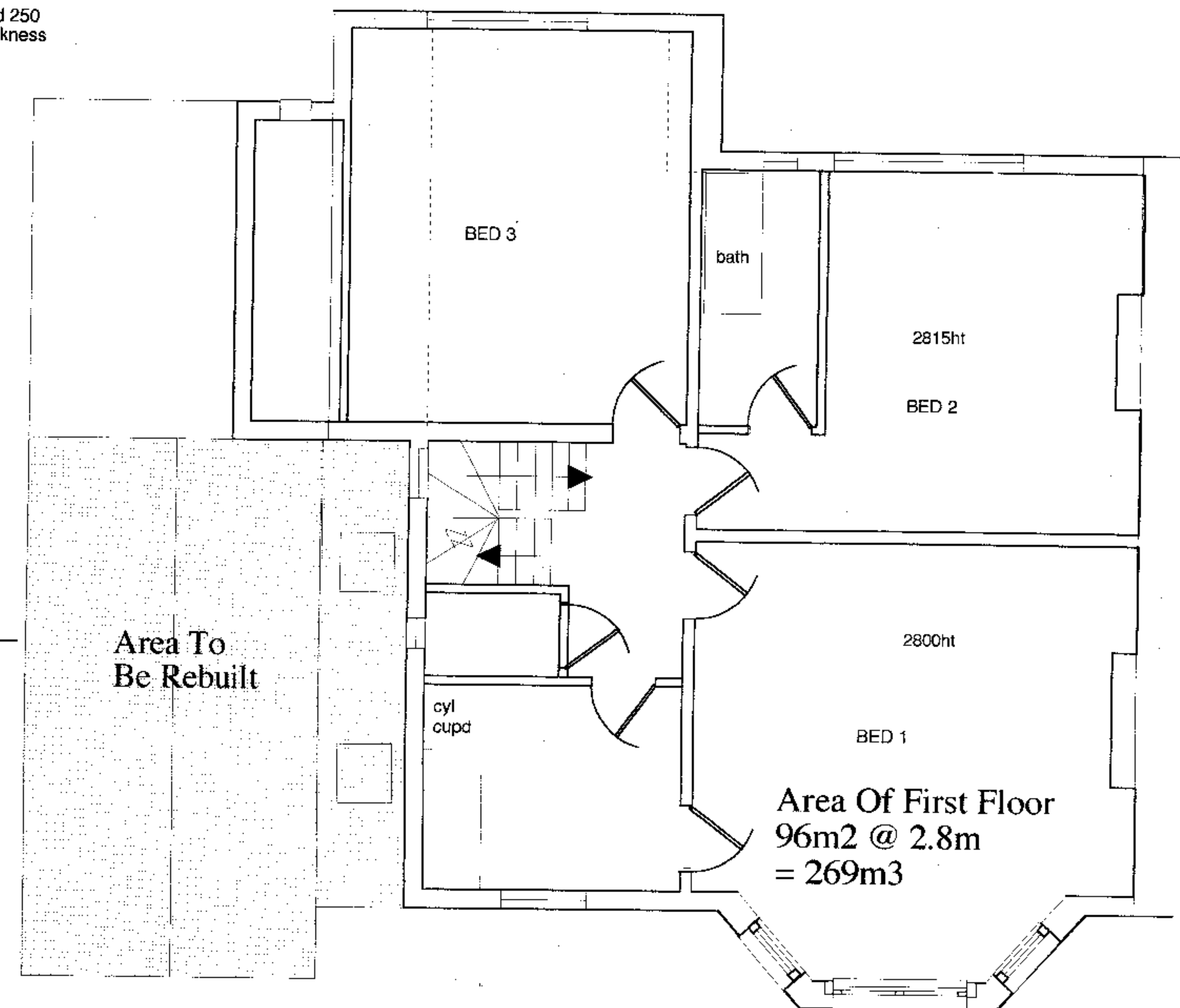
FIRST FLOOR
