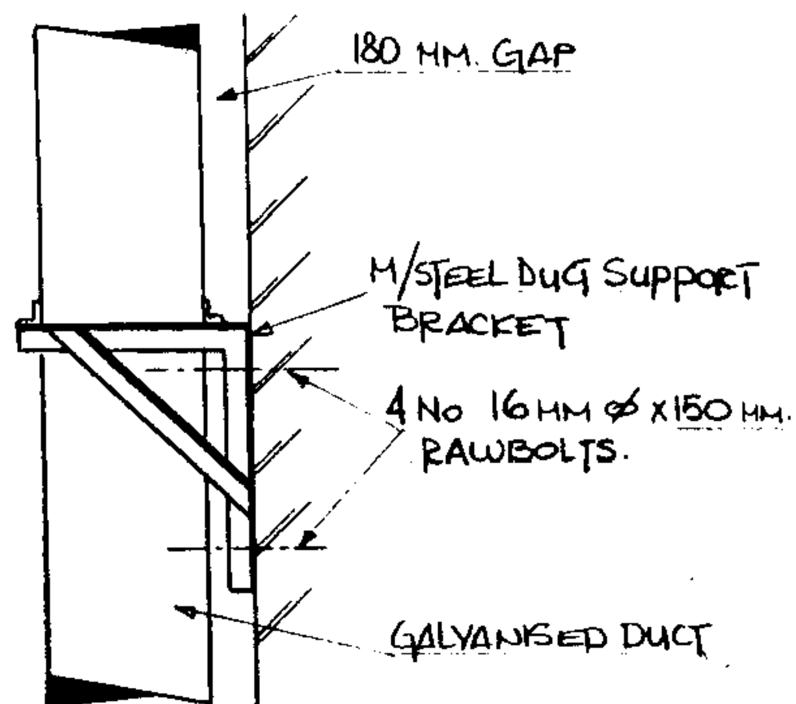
DETAIL OF DUCT BRACKET (NTS)
