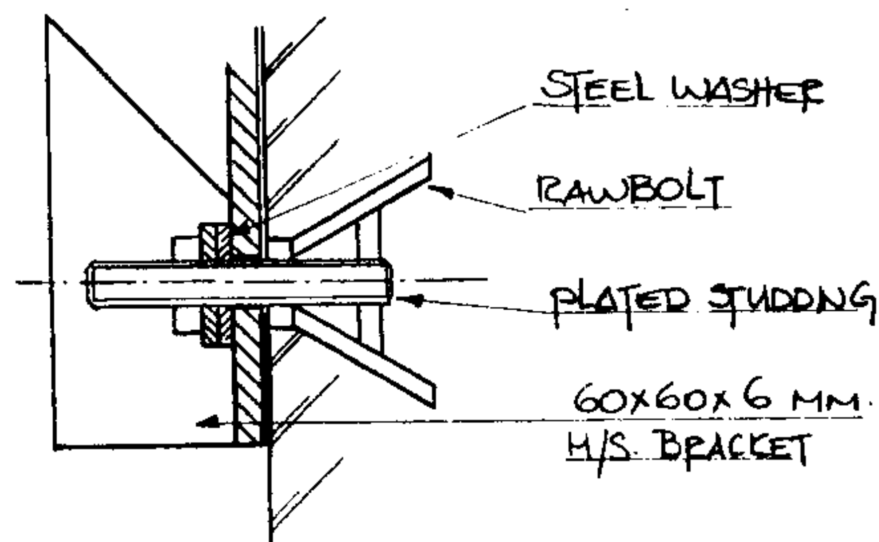
DETAIL OF BRACKET FIXING (NTS.)
