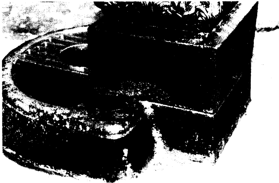
figure 26. Corrosion to base of cast iron drinking fountain
