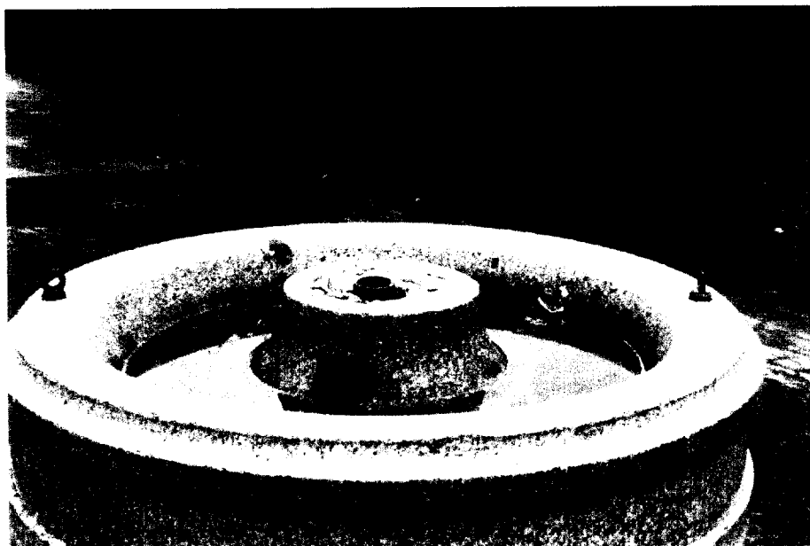
figure 23 . Missing Upper Spout feature to granite drinking fountain
