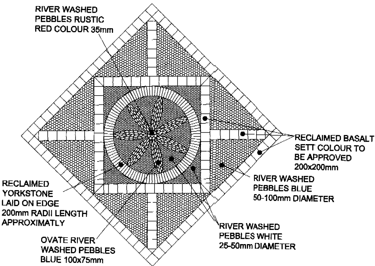
DETAIL B SCALE 1:50
