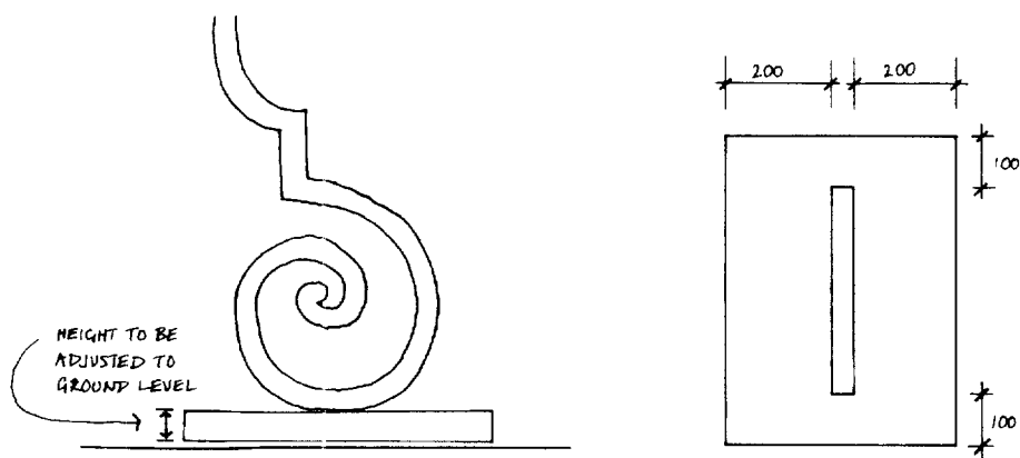
figure 7. Proposed cross section and plan of hidden coiled backstay at Highgate Hill Entrance
