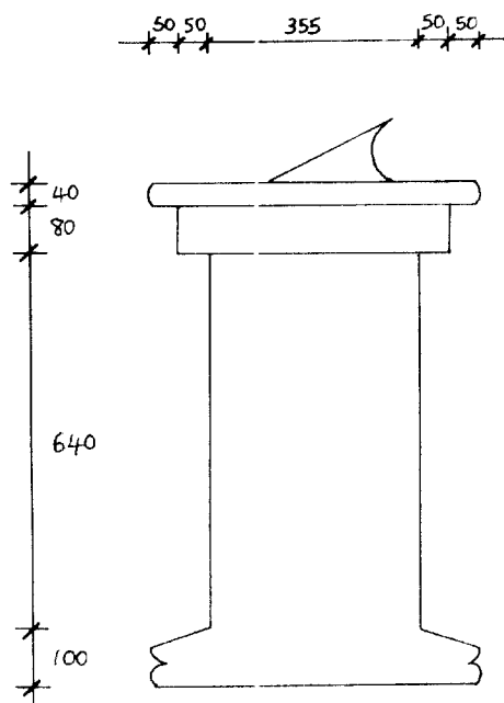
figure 31. Cross Section of Small Sundial. Approximate dimensions.
