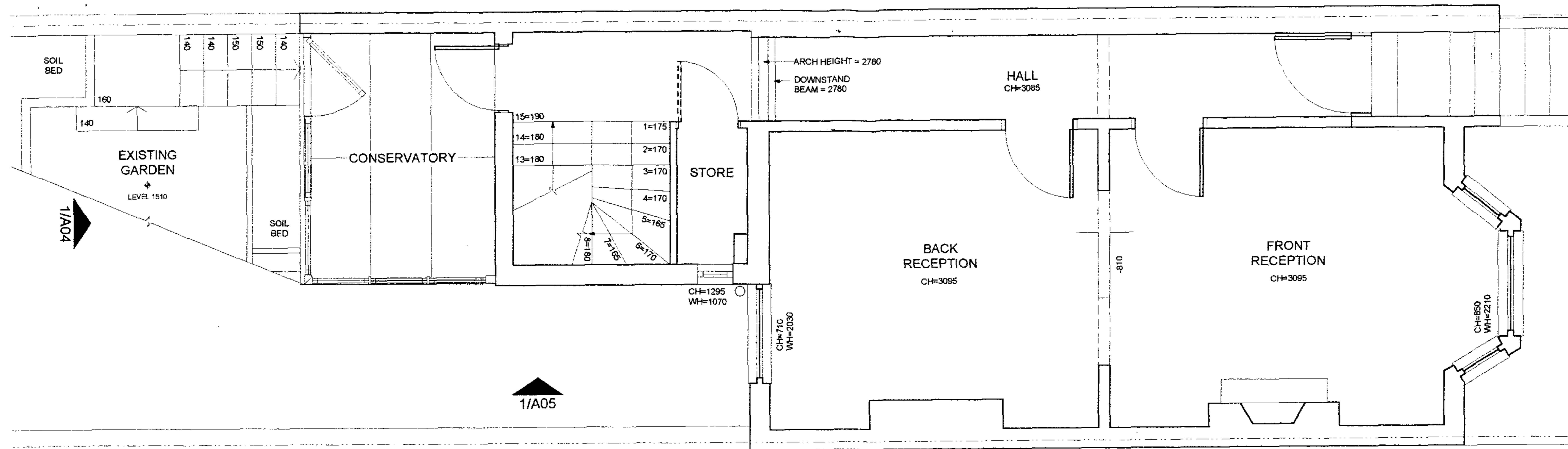
2 UPPER GROUND FLOOR 1:50
