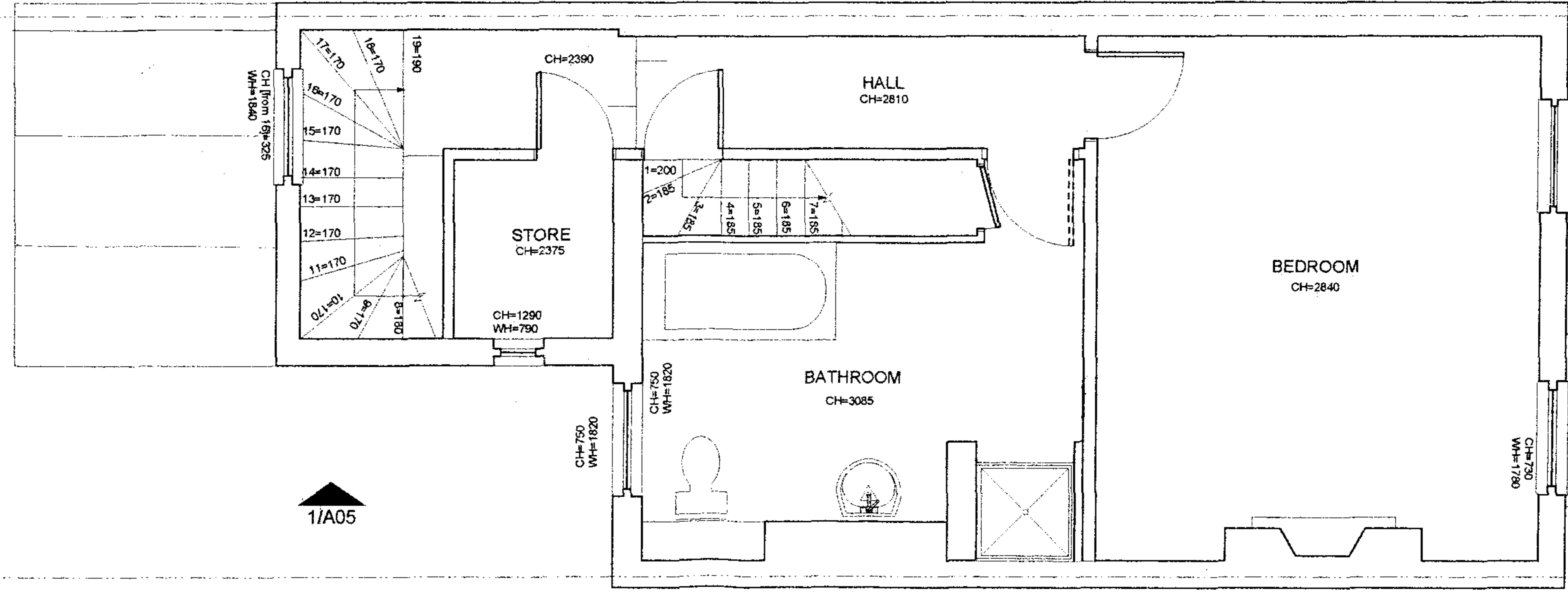
1 FIRST FLOOR 1:50
