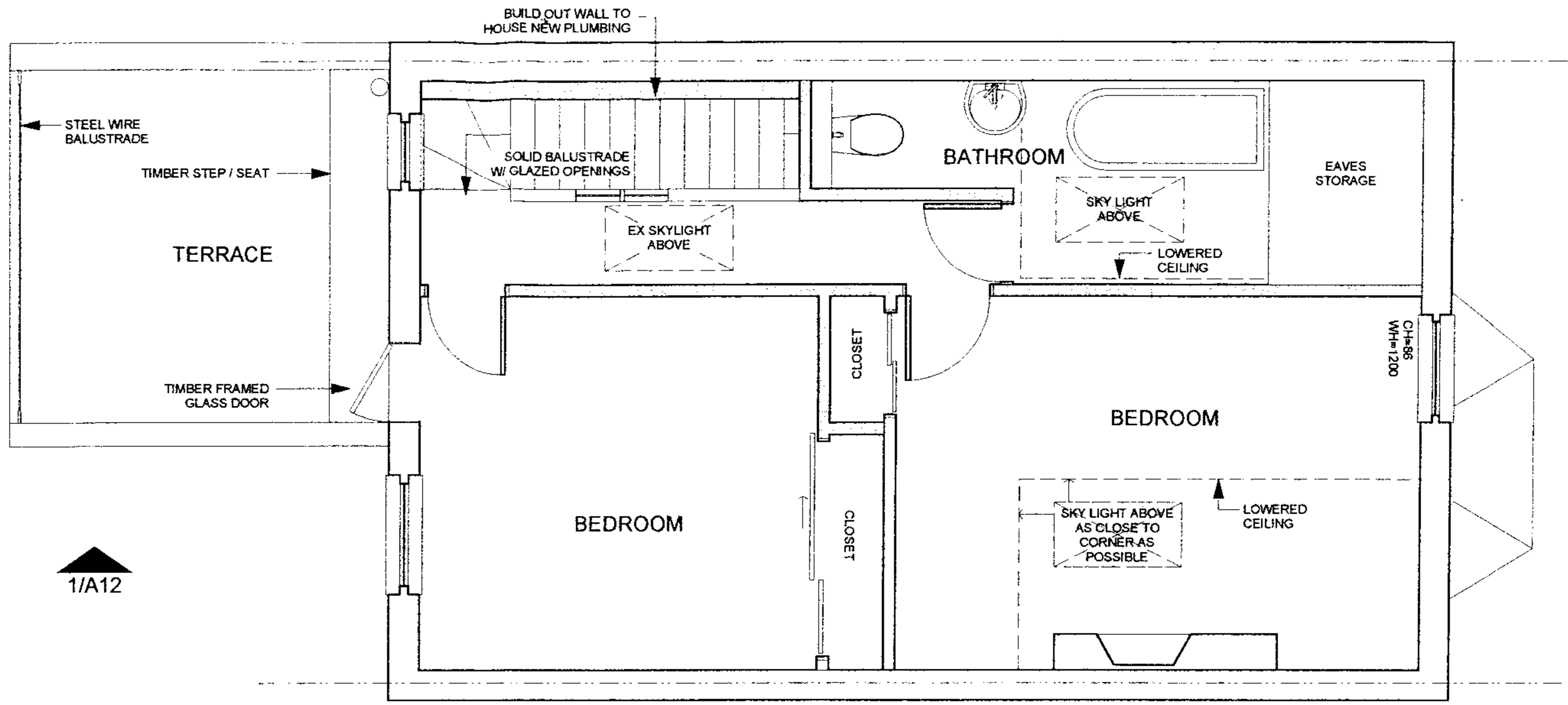
2 SECOND FLOOR 1:50
