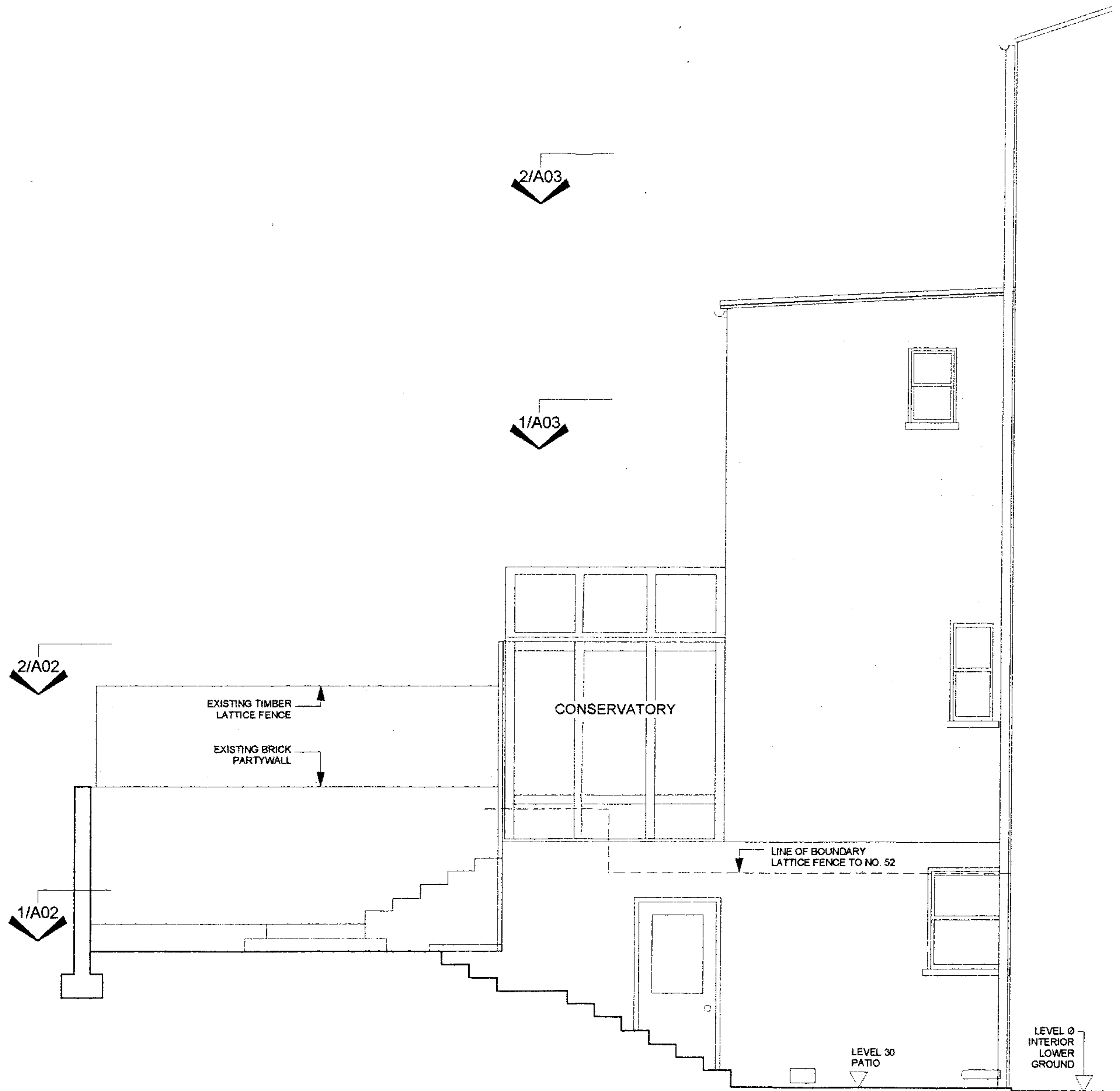
1 EXISTING SIDE ELEVATION 1:50
