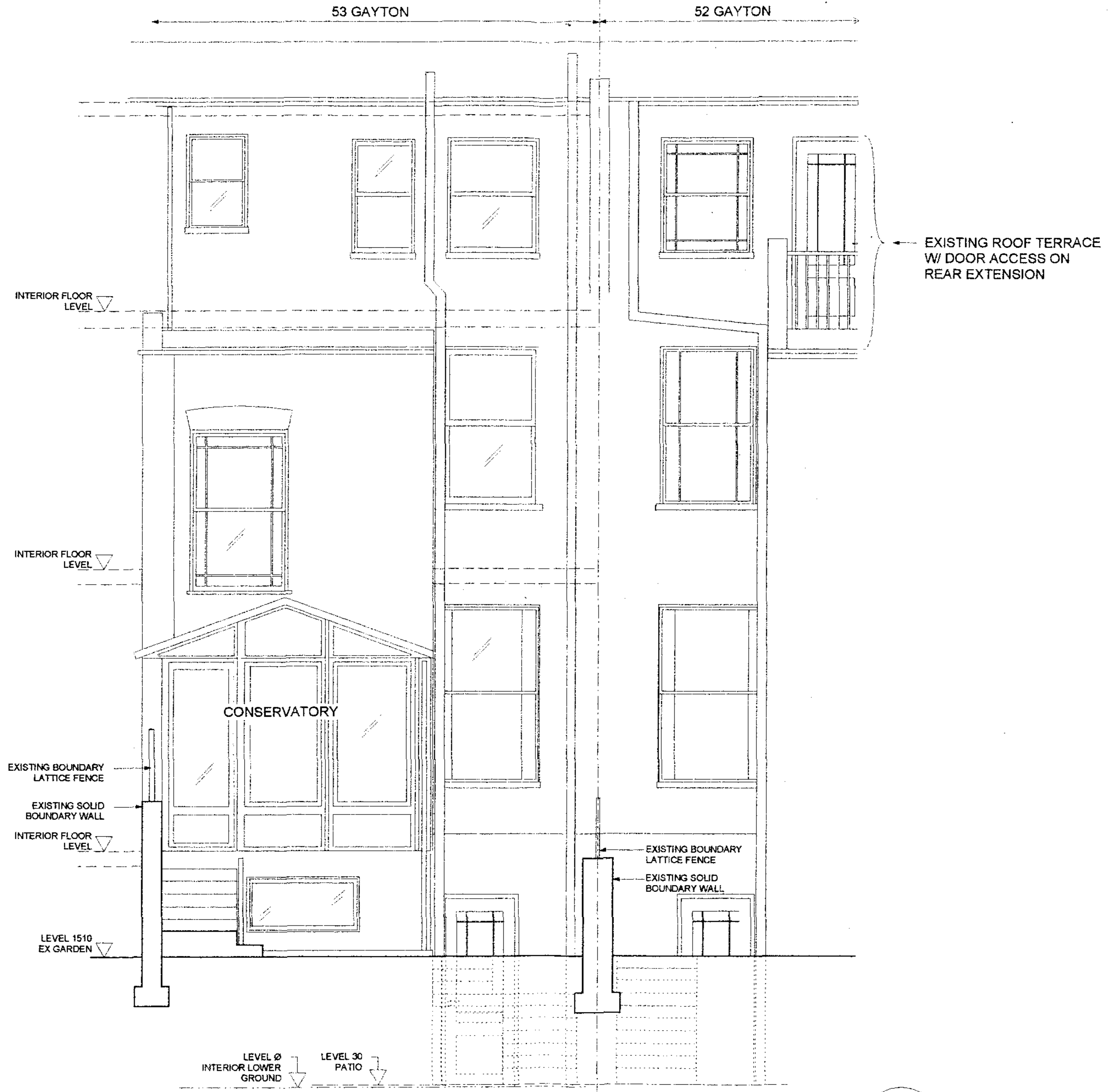
EXISTING REAR ELEVATION 1:50
