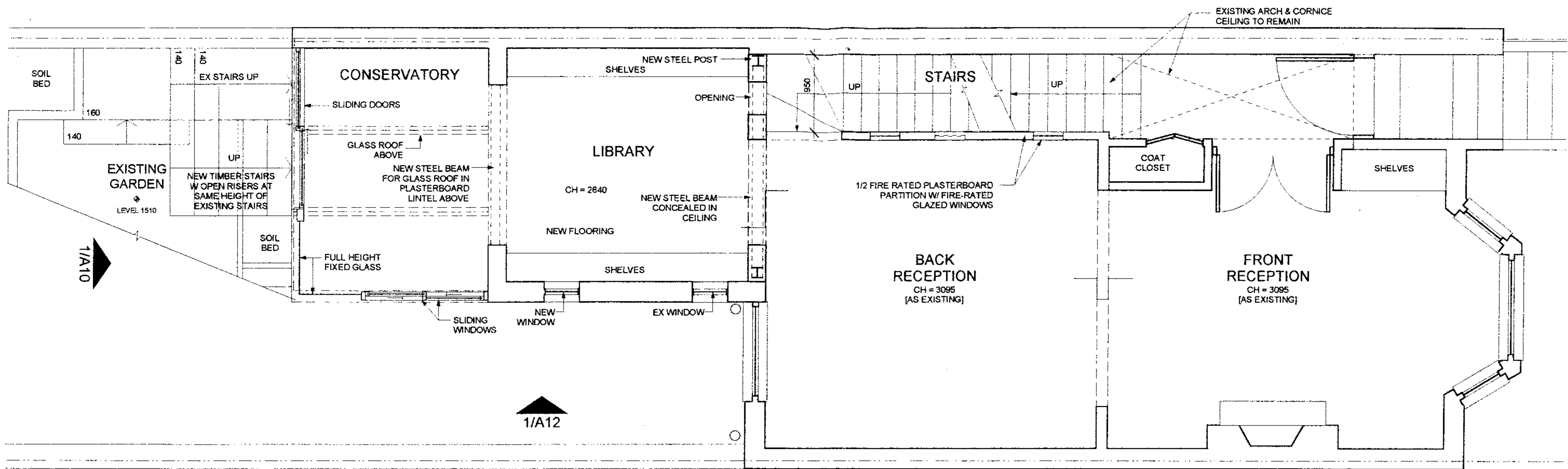
2 UPPER GROUND FLOOR 1:50
