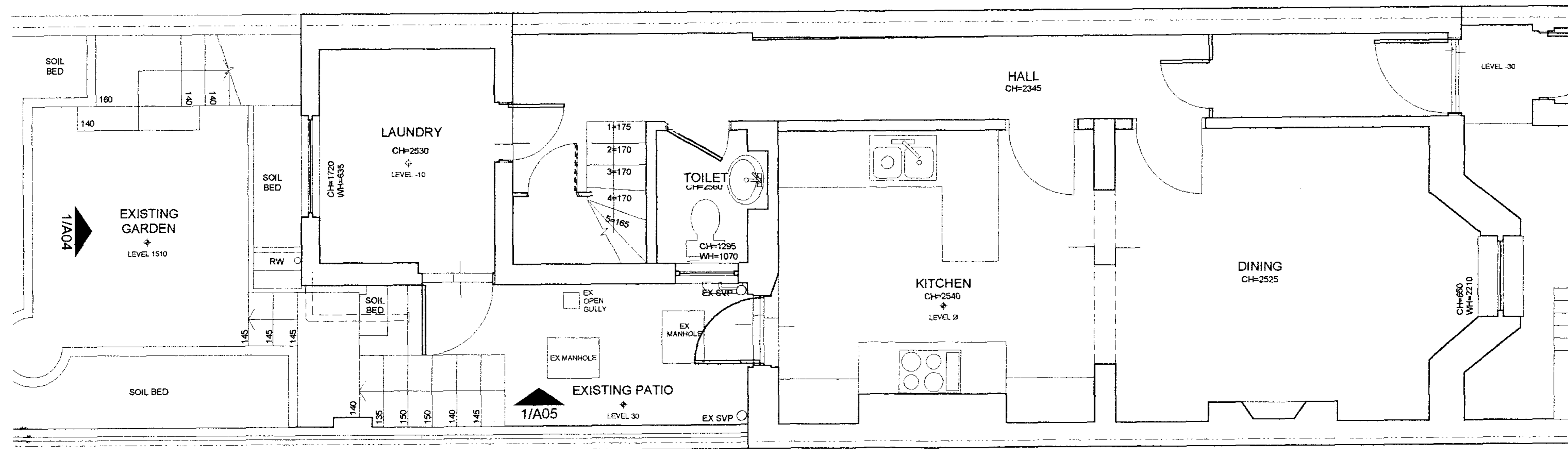
1 LOWER GROUND FLOOR 1:50
