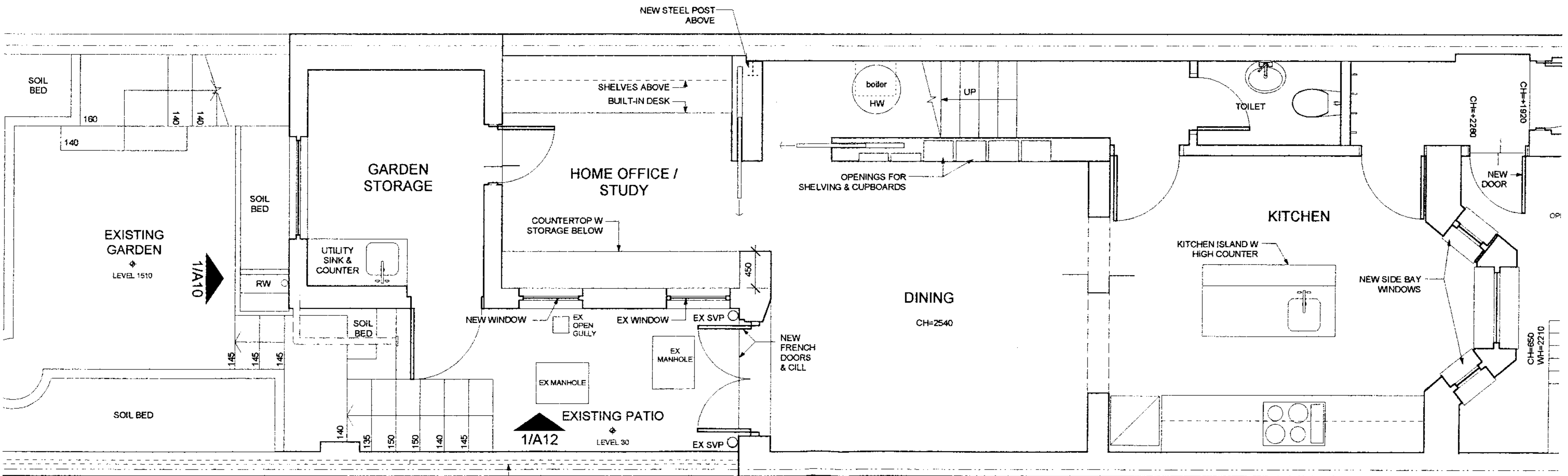
1 LOWER GROUND FLOOR 1:50
