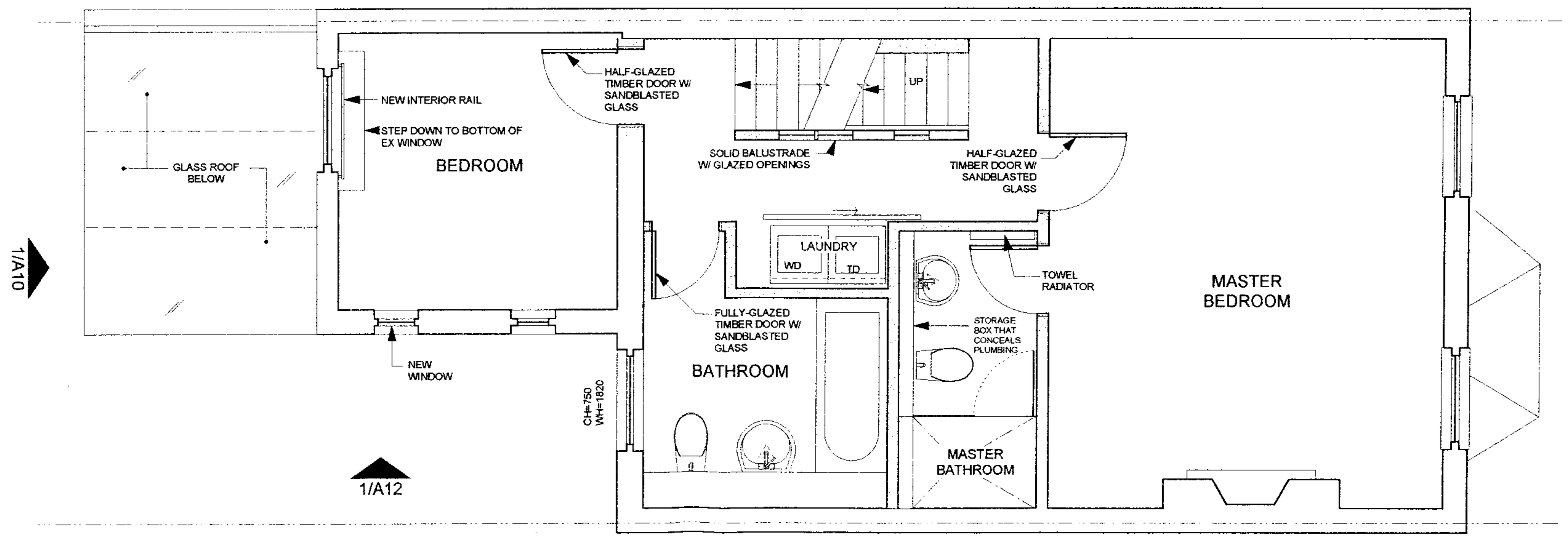
1 FIRST FLOOR 1:50
