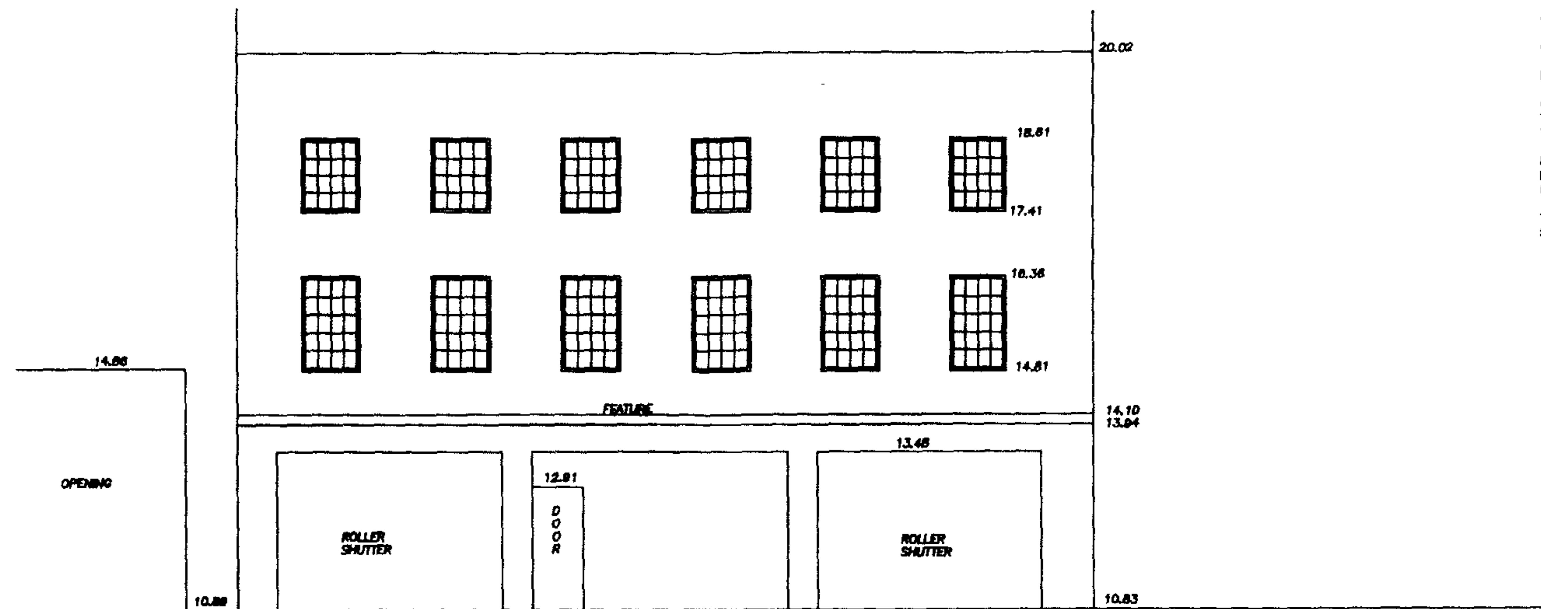
EXISTING FRONT ELEVATION
