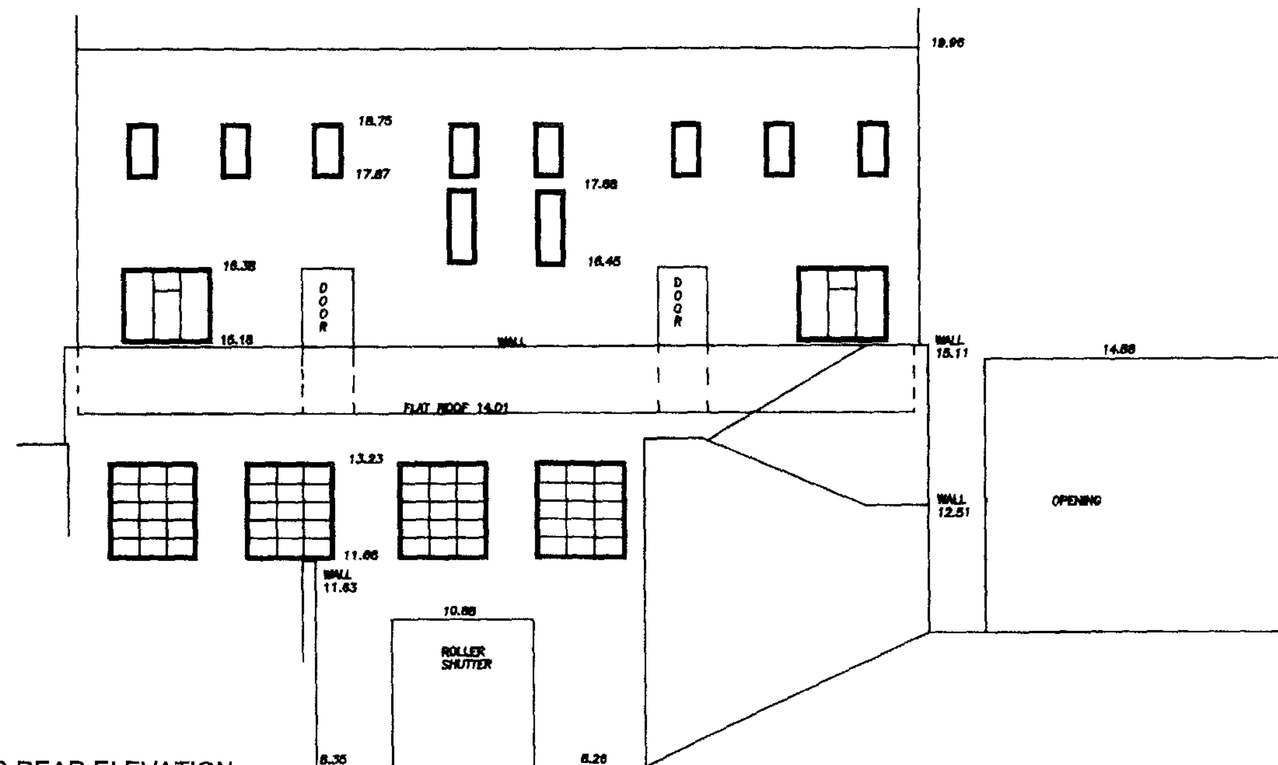
EXISTING REAR ELEVATION
