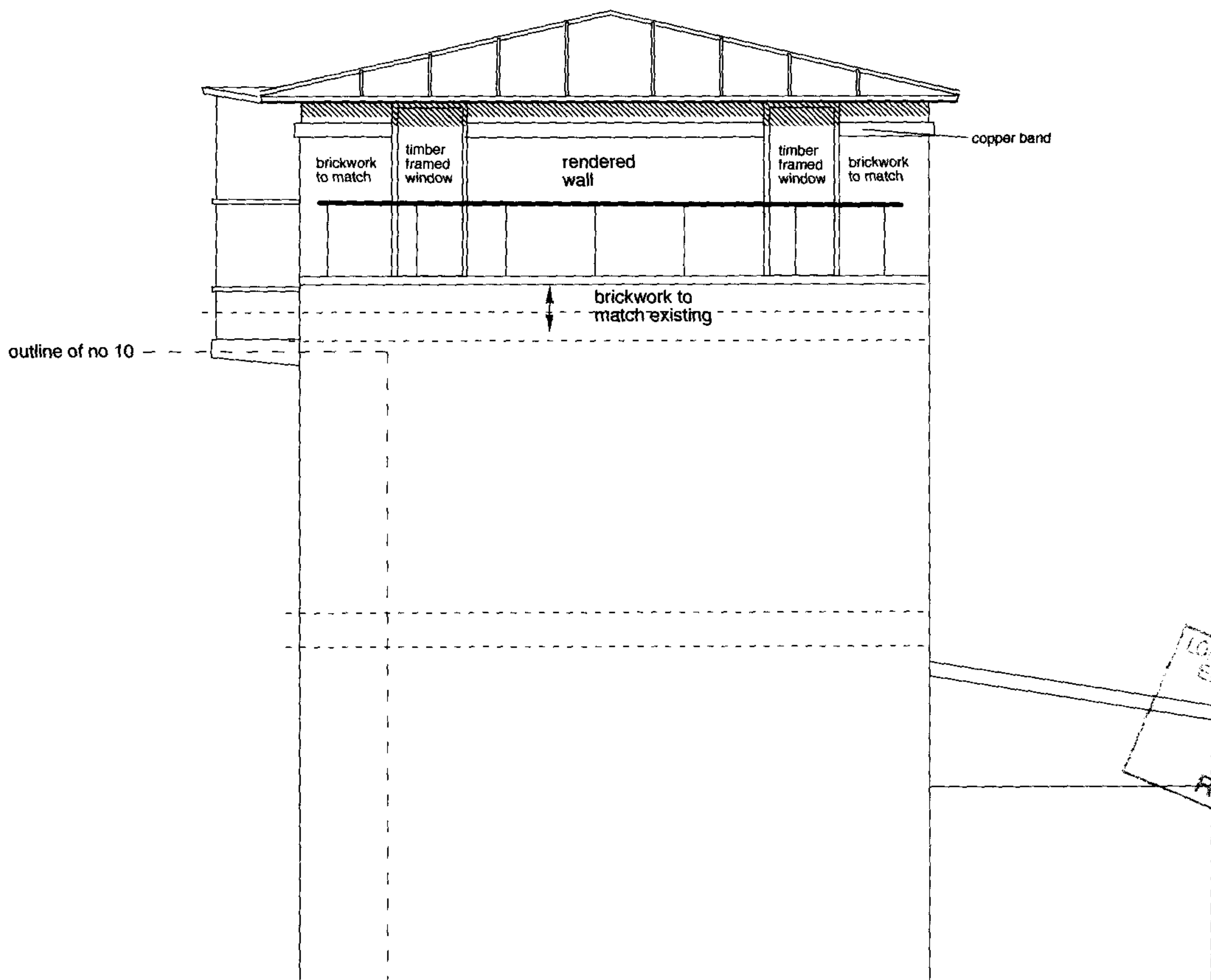
REAR ELEVATION
