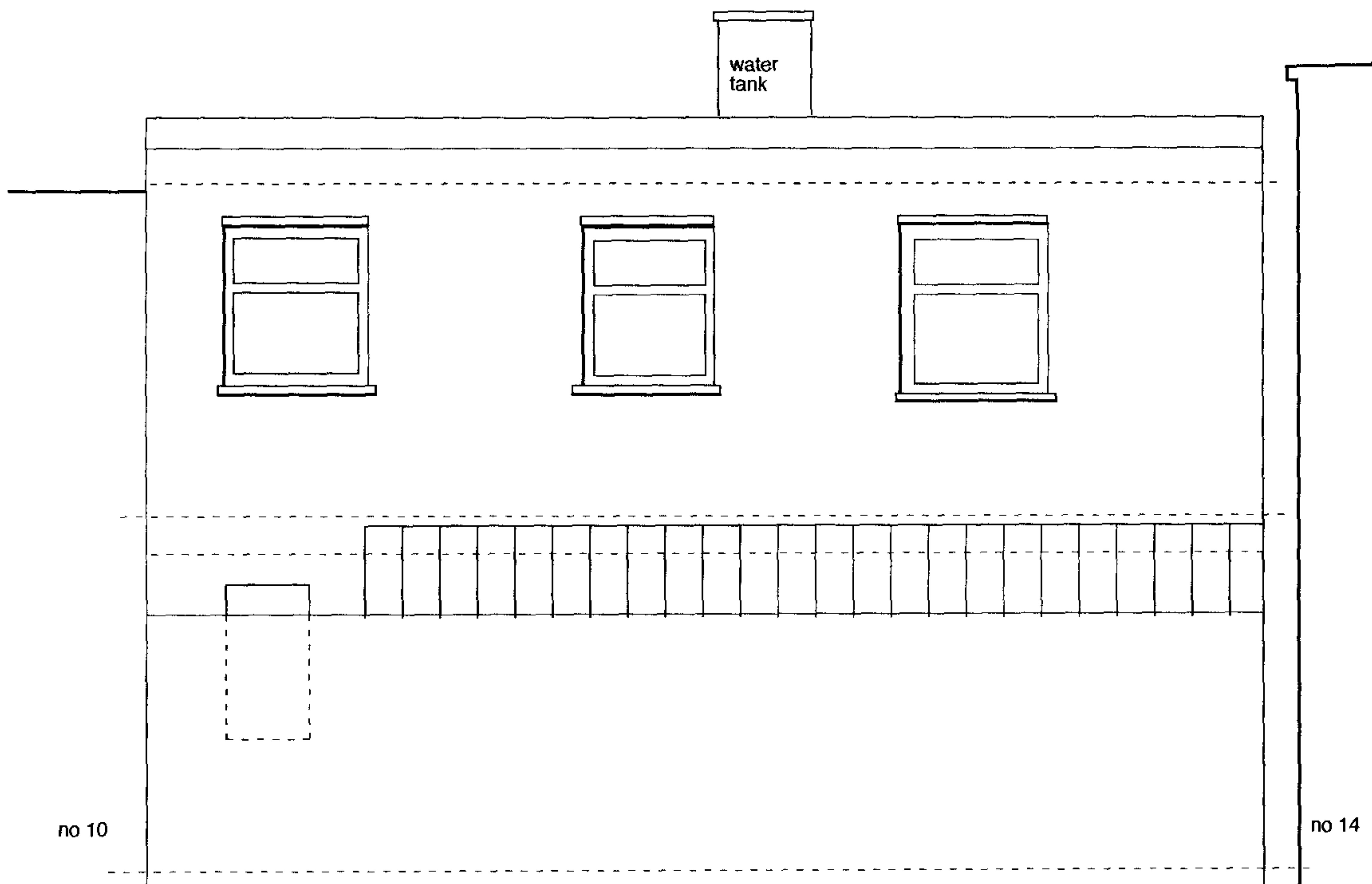
FRONT ELEVATION
