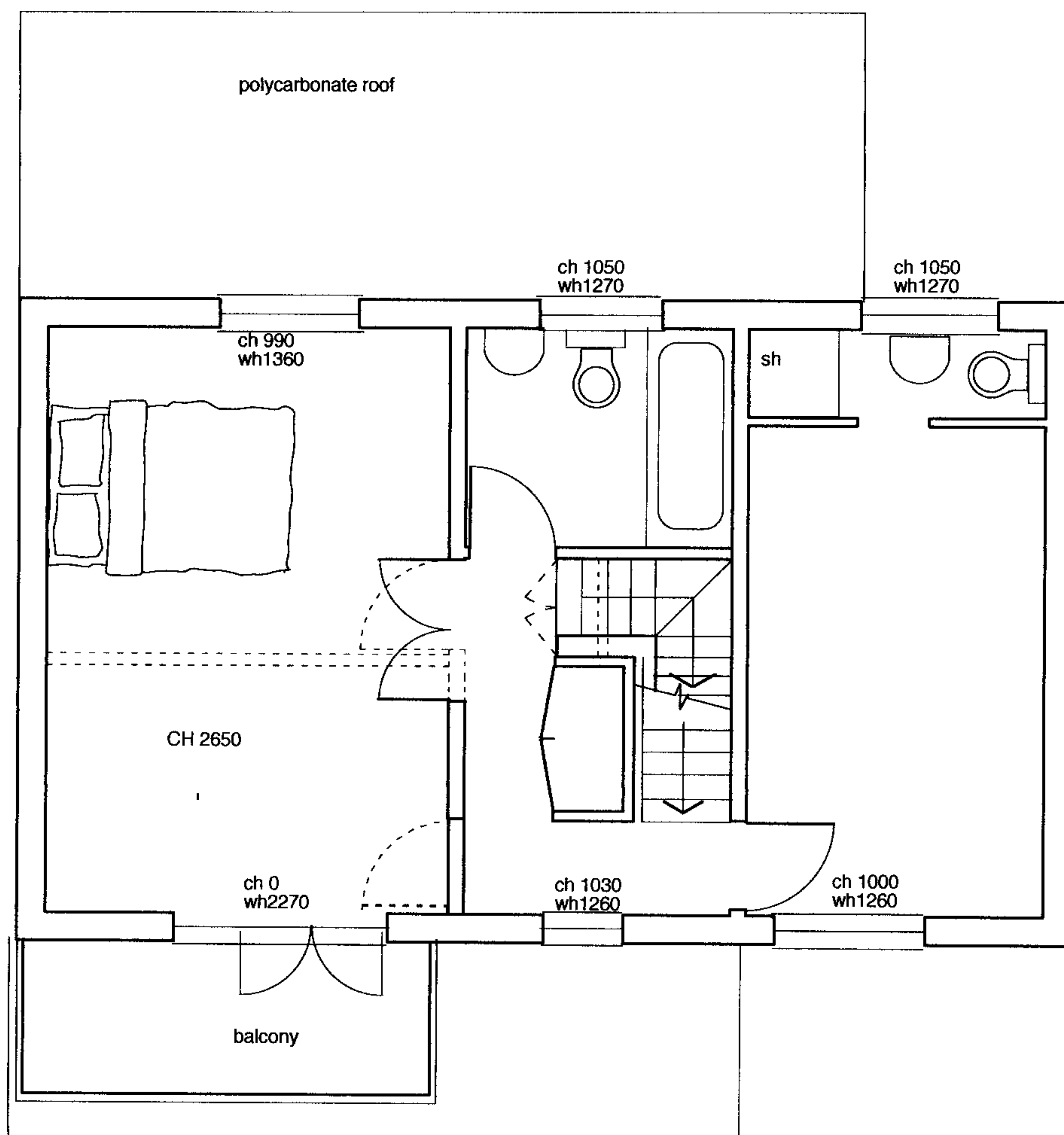
1ST FLOOR
