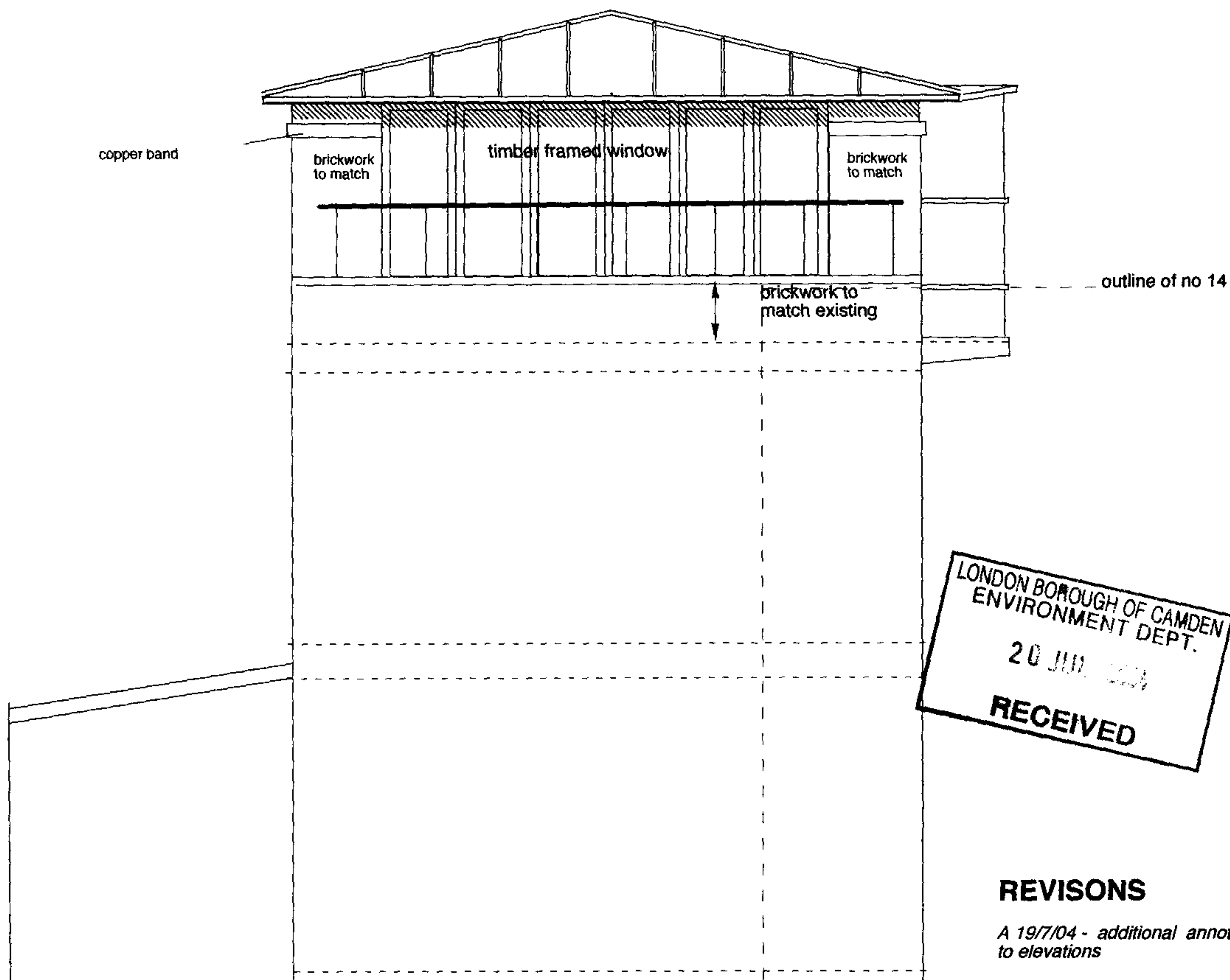
NORTH EAST ELEVATION
