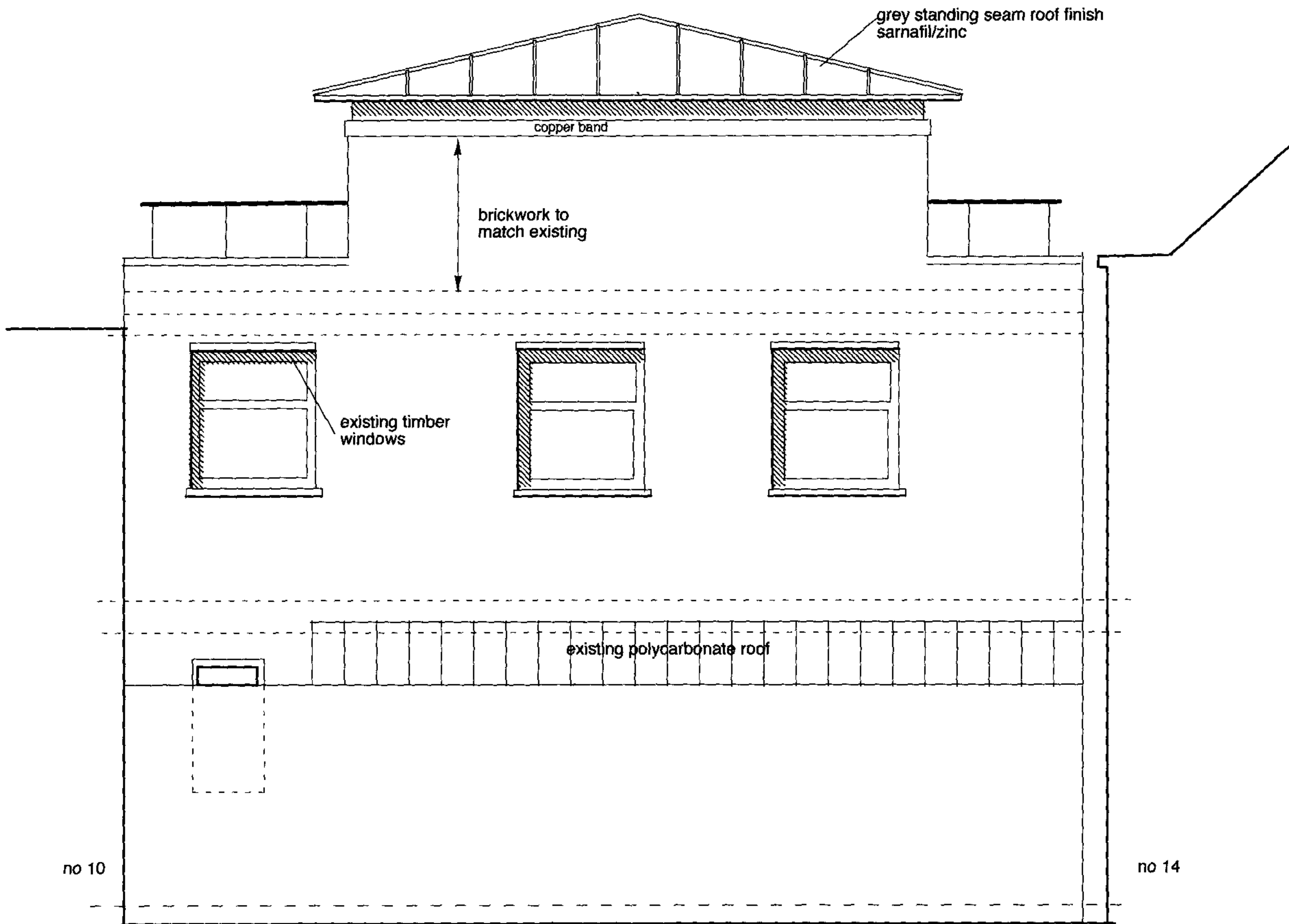
REAR ELEVATION
