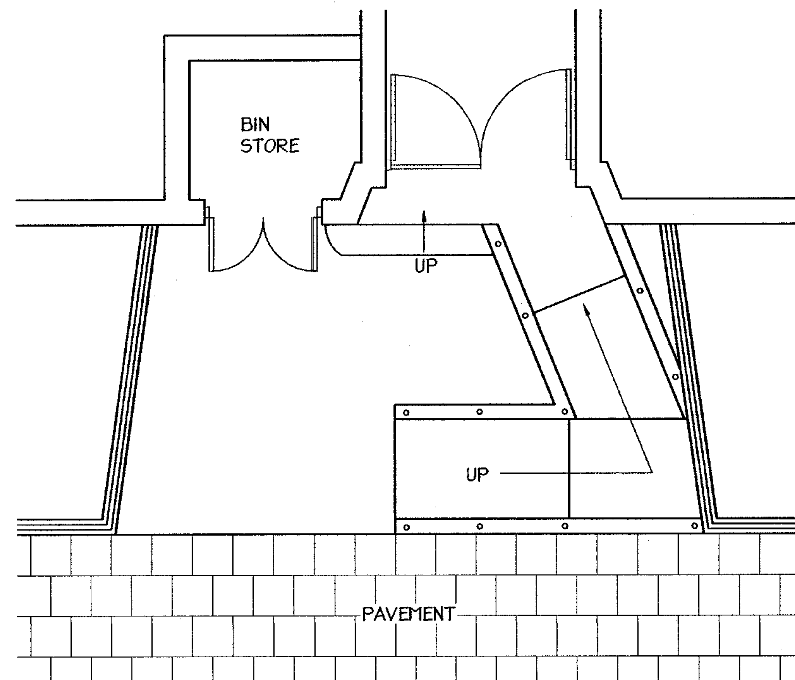
PROPOSED PLAN
