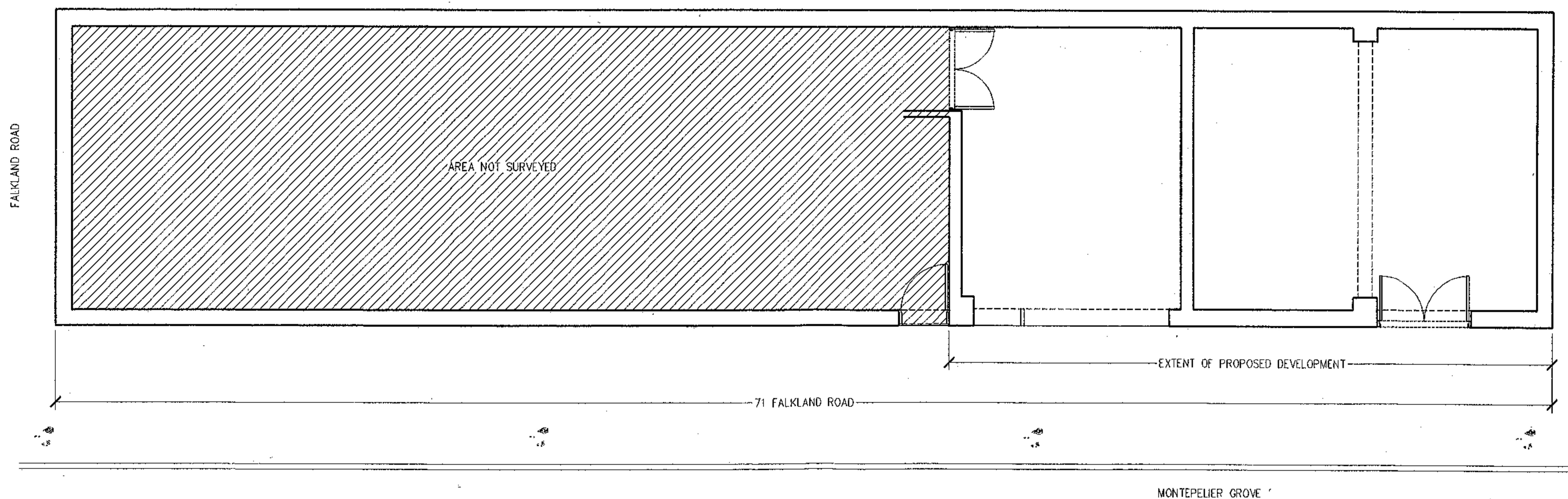
EXISTING GROUND FLOOR PLAN 1:100
