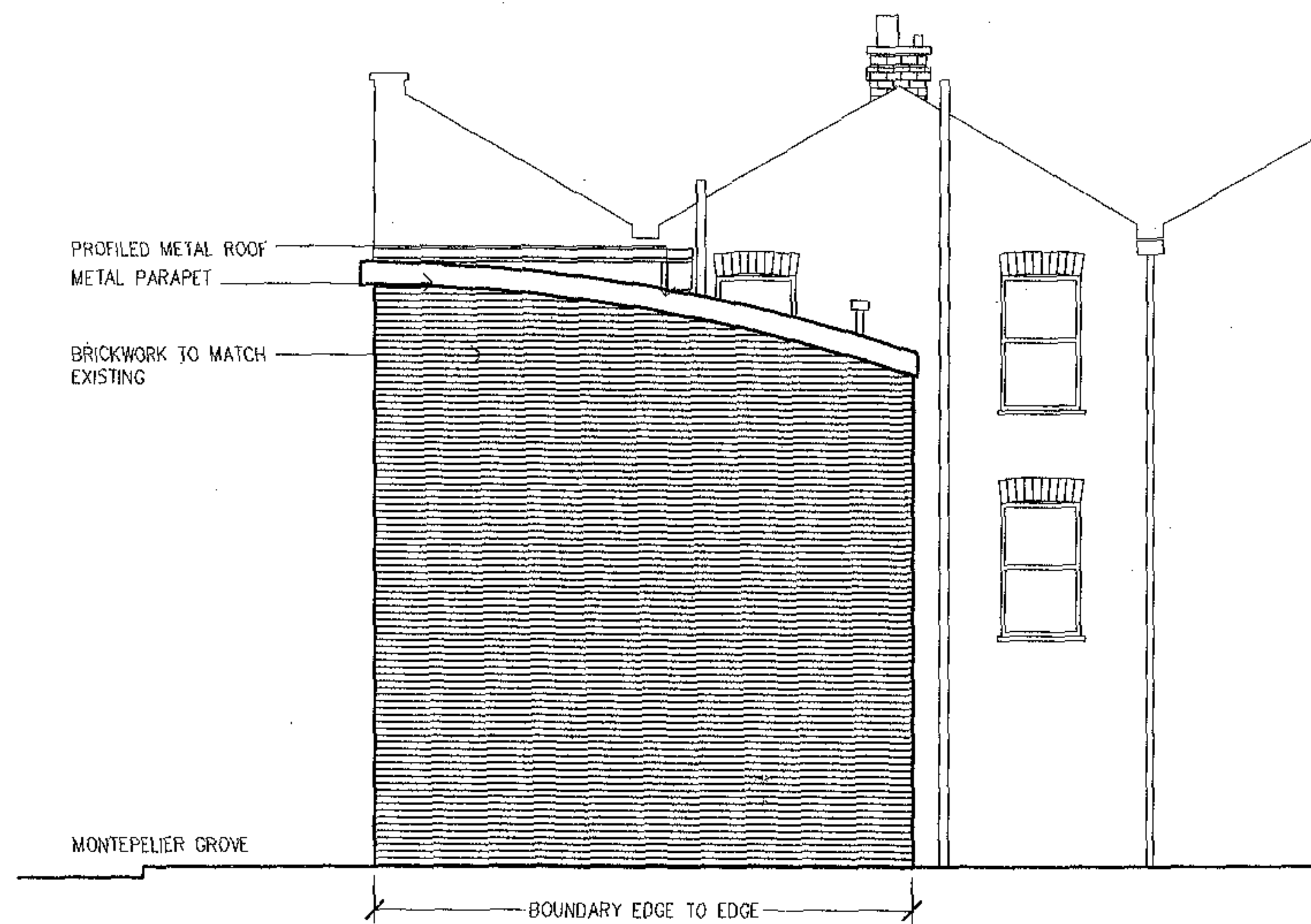
PROPOSED SIDE ELEVATION 1:100
