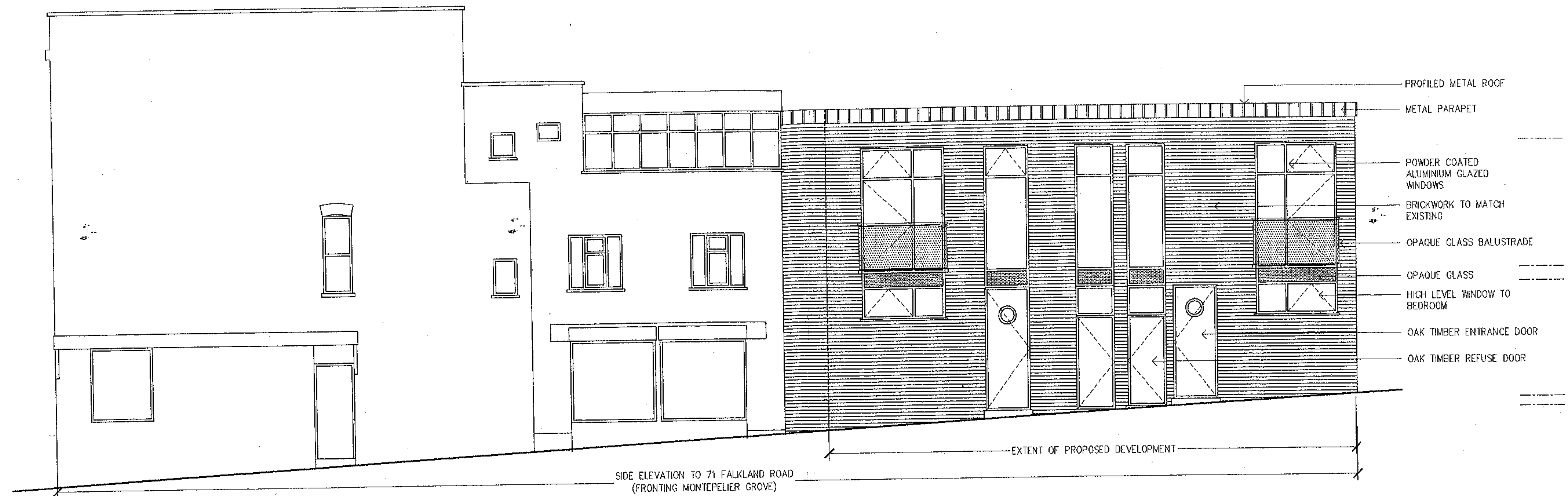
PROPOSED FRONT ELEVATION 1:100
