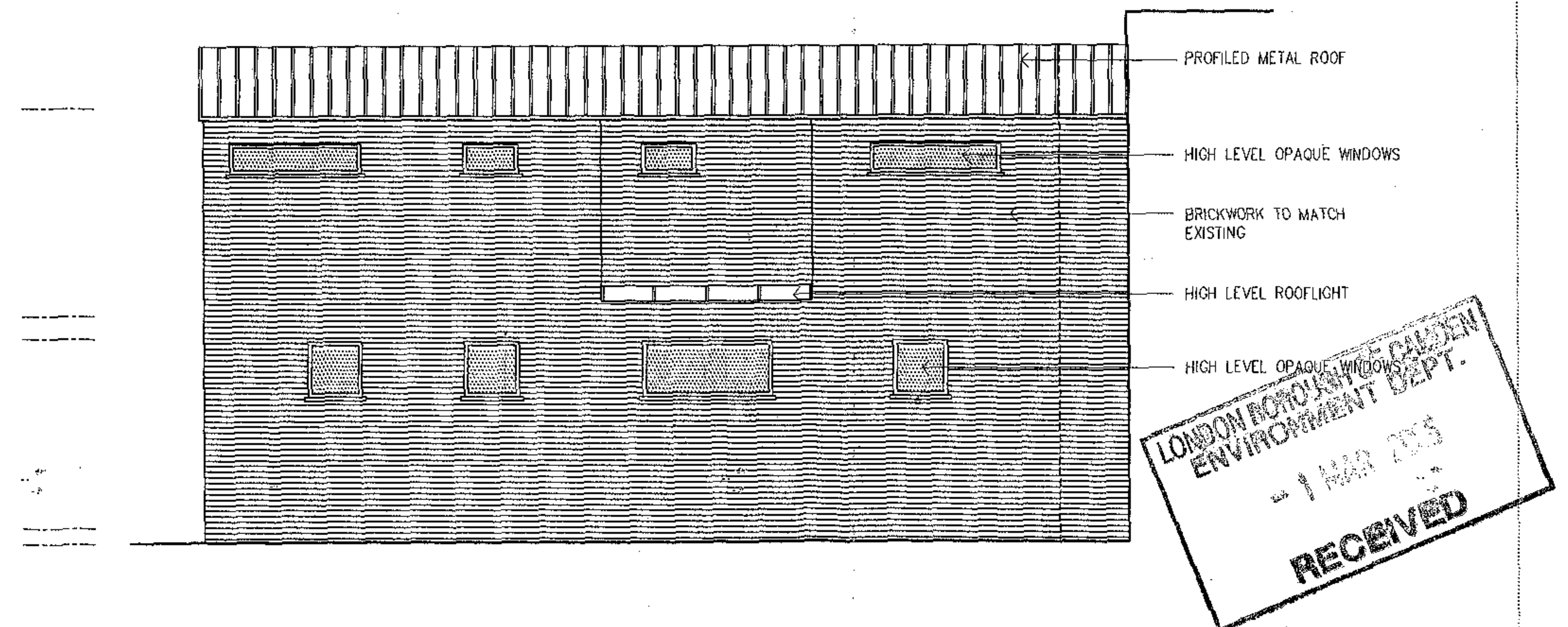
PROPOSED REAR ELEVATION 1:100
