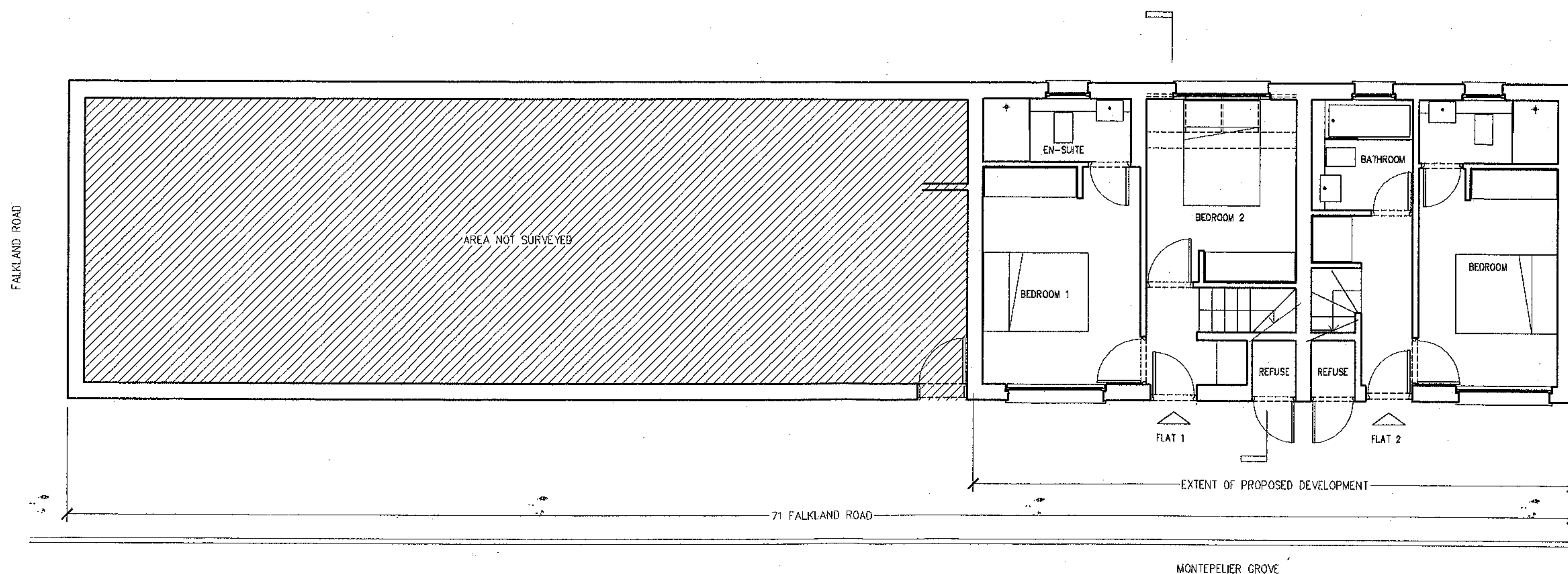
PROPOSED GROUND FLOOR PLAN 1:100
