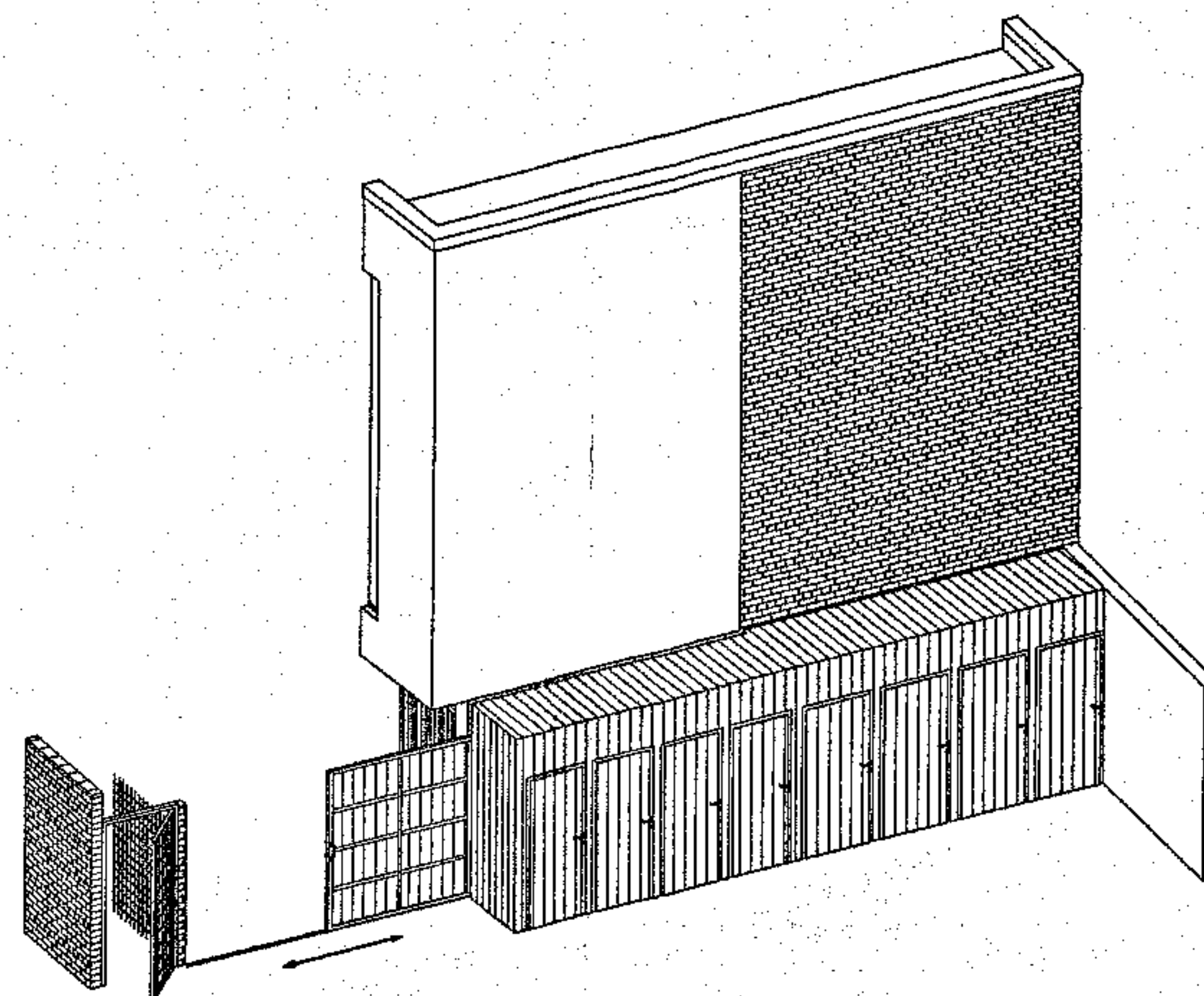
Gate in half open position
