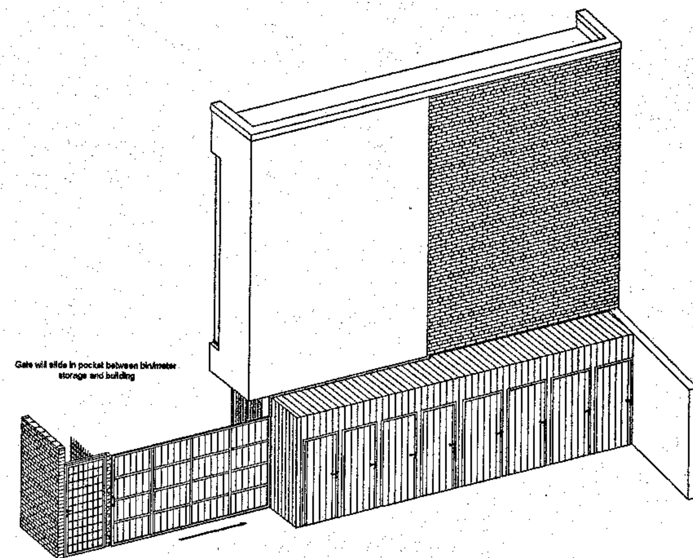
Gate in closed position
