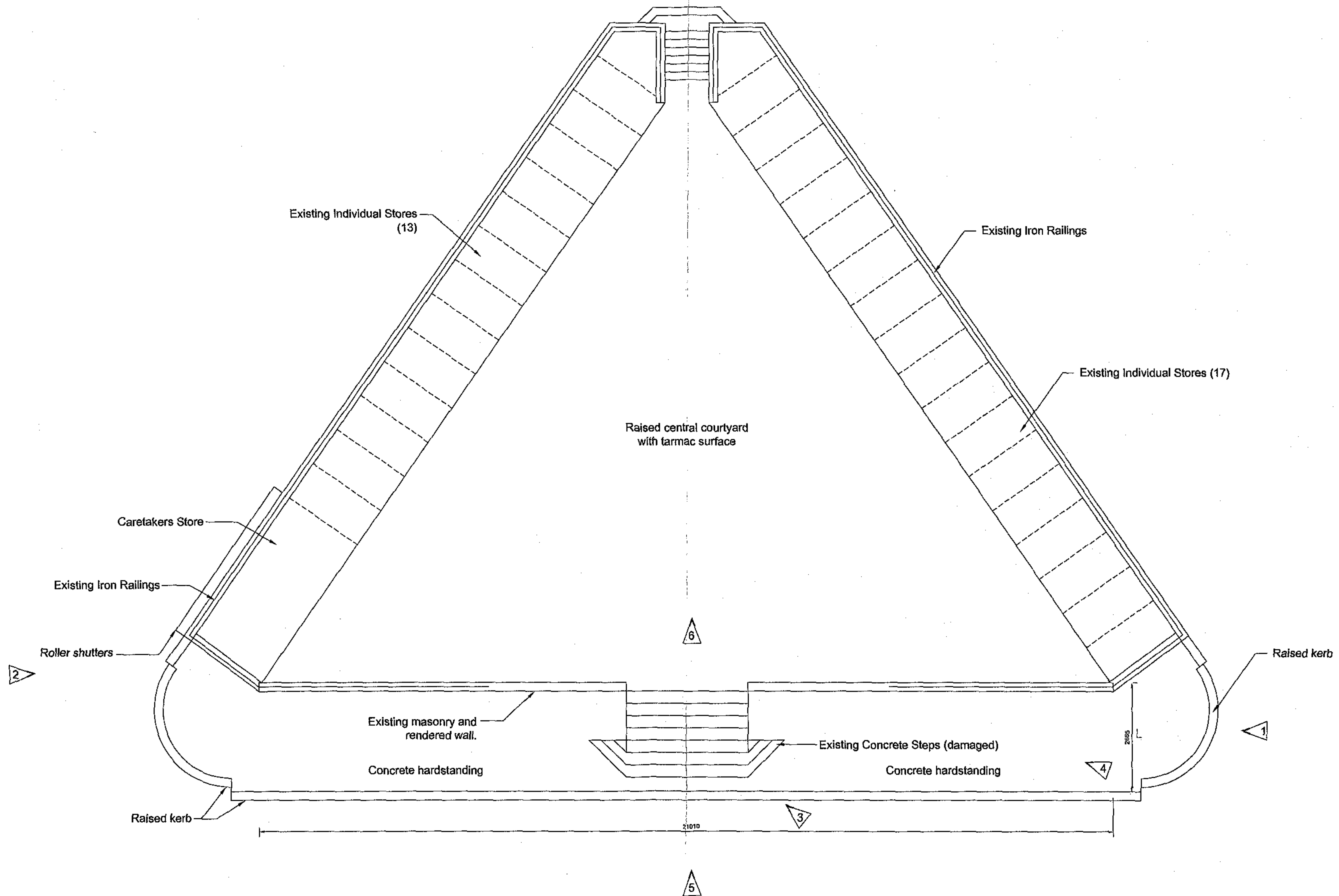
Existing Plan
