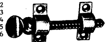
SASH SCREW BRASS Head and Plates. Mild STEEL Shank. Dia. 8mm
