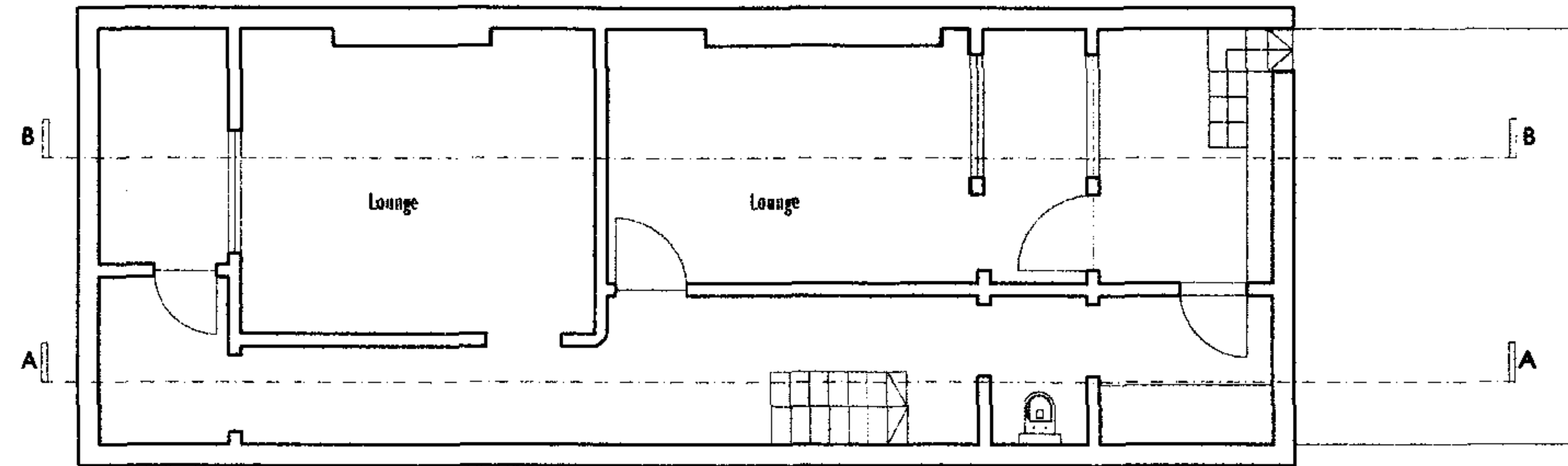
Existing Basement Plan
