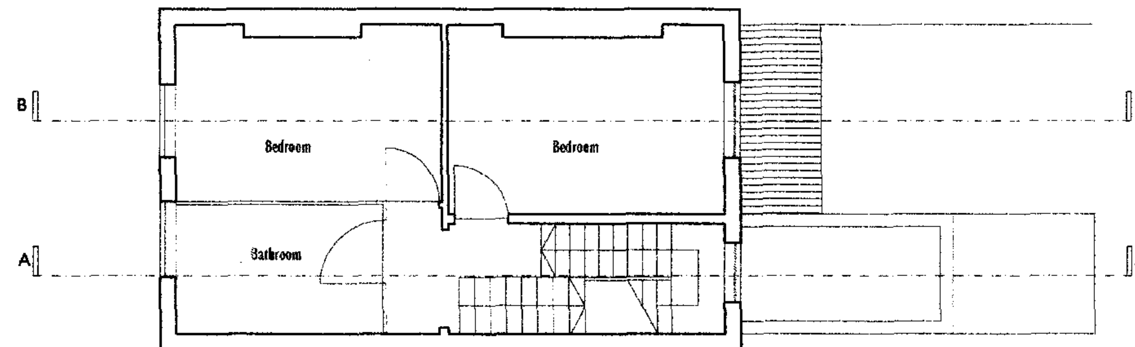
Existing Second Floor Plan
