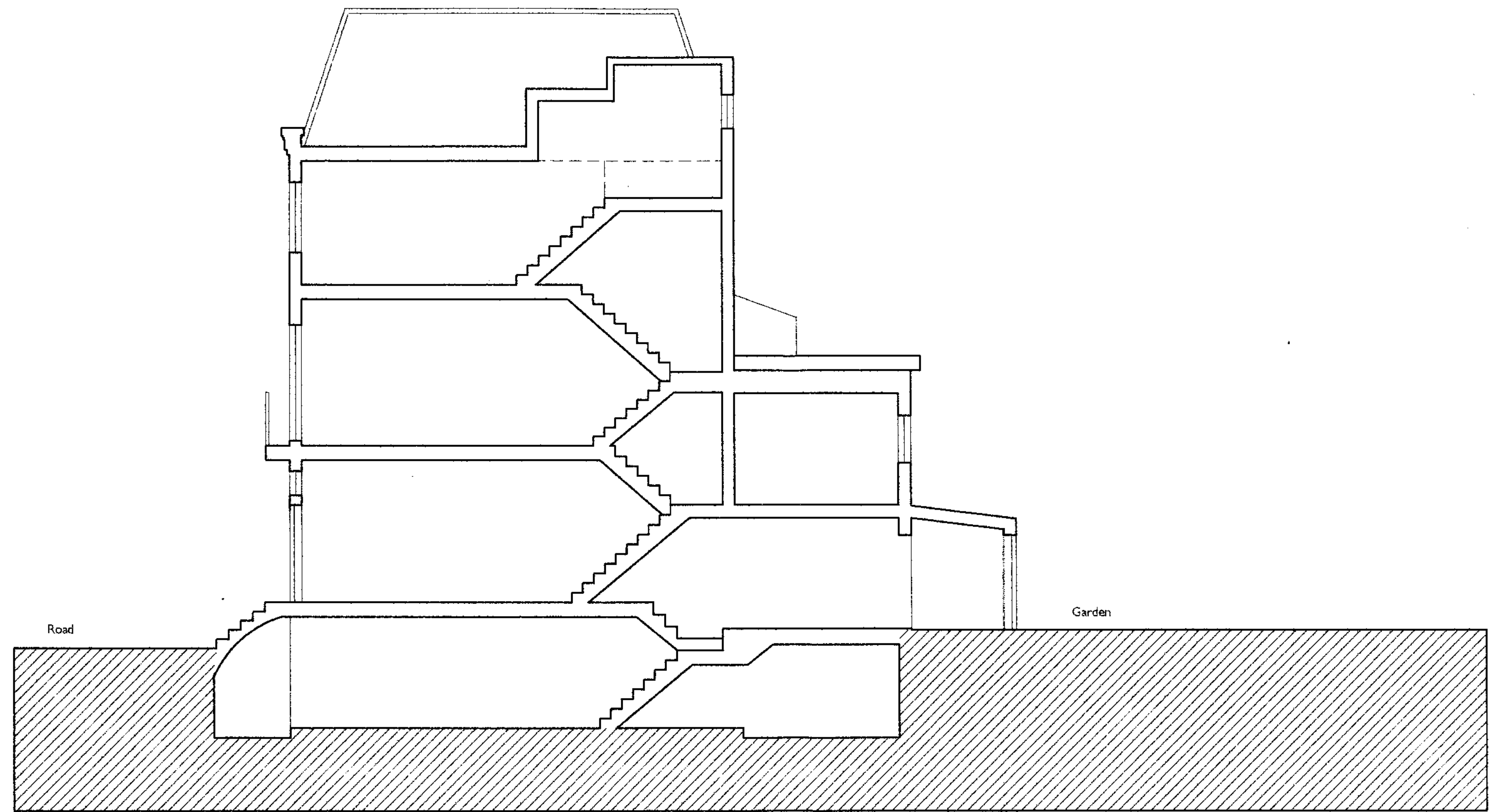
Existing Section AA
