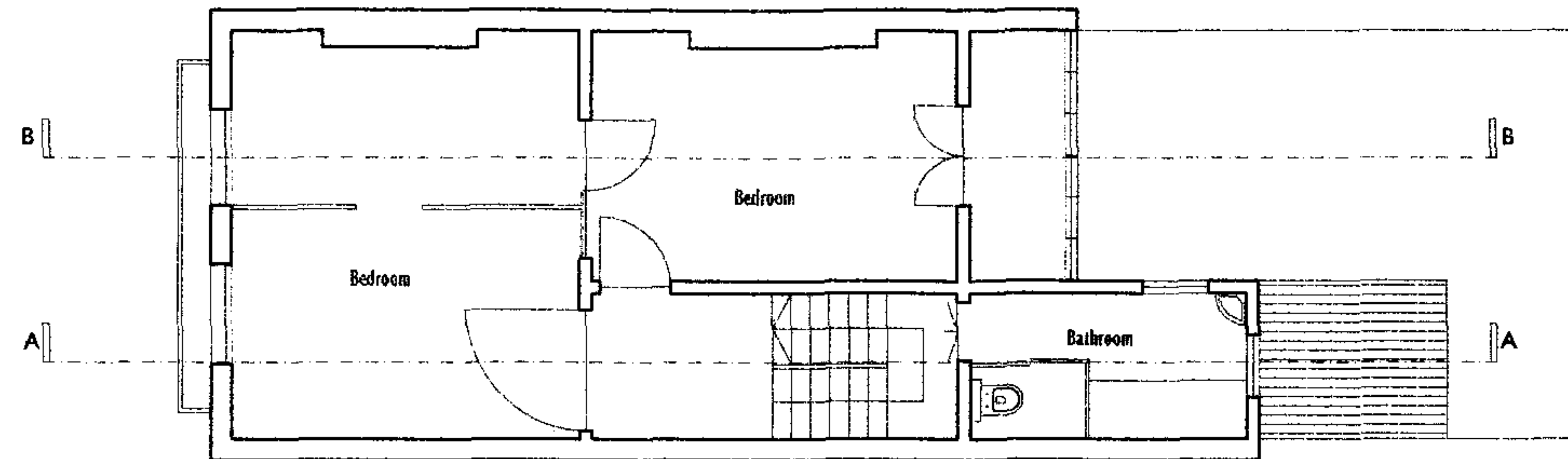
Existing First Floor Plan
