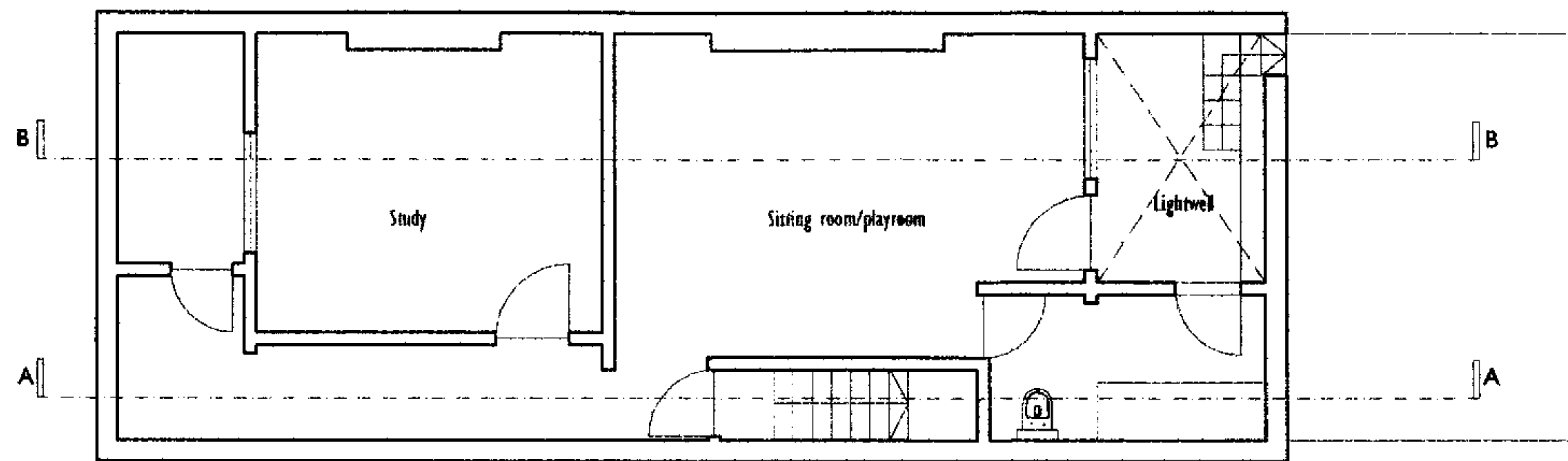
Proposed Basement Plan
